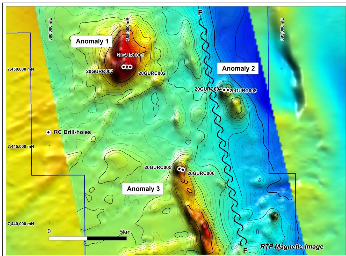
Figure 1: Gunanya Prospect showing RC drill-holes relative to magnetic targets
