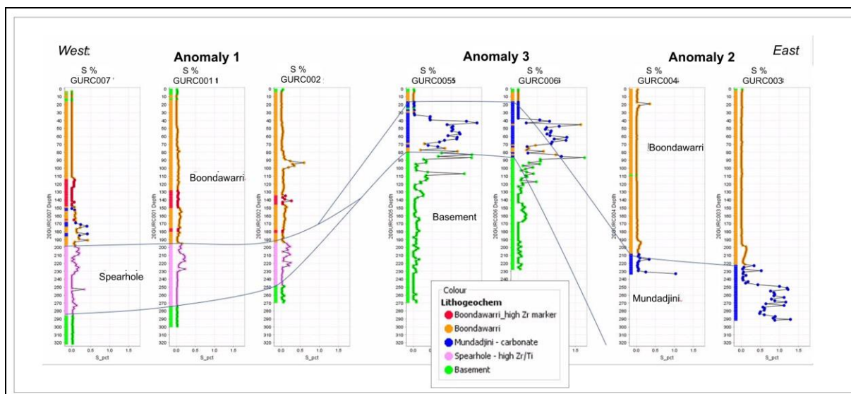
Figure 2: Gunanya RC drill-holes showing variation in sediments across the project
