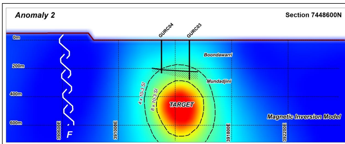
Figure 3: Gunanya Anomaly 2 magnetic inversion model showing drill hole locations
