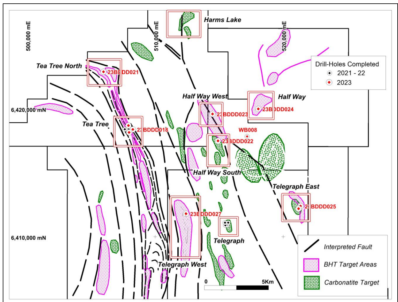
Figure 4: Balladonia Project showing BHT and carbonatite target areas interpreted from aeromagnetic data.
