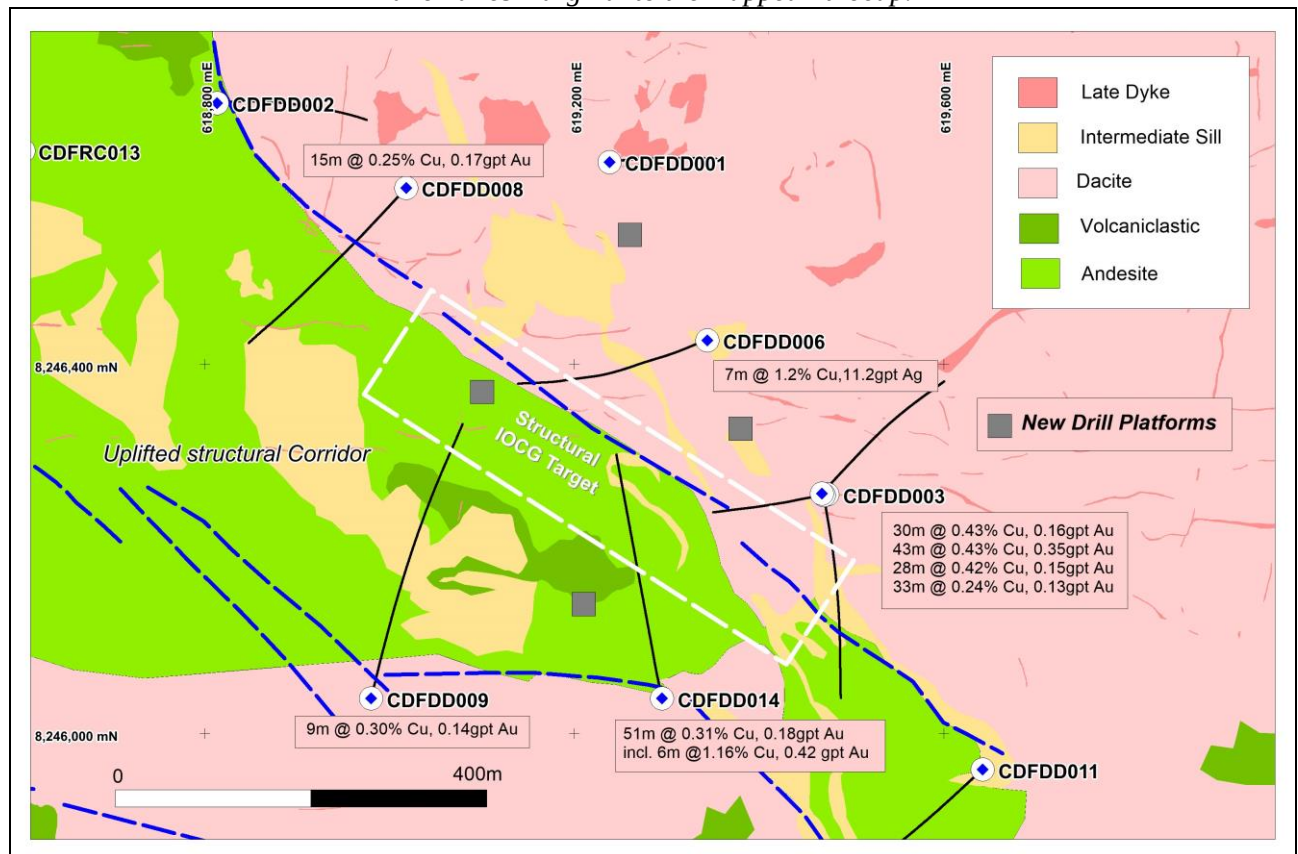
Figure 10: Cerro de Fierro Prospect showing location of the structural target and new drilling platforms. Drill results on the plan were previously reported to the ASX on 19 December 2018 and 5 March 2020.
