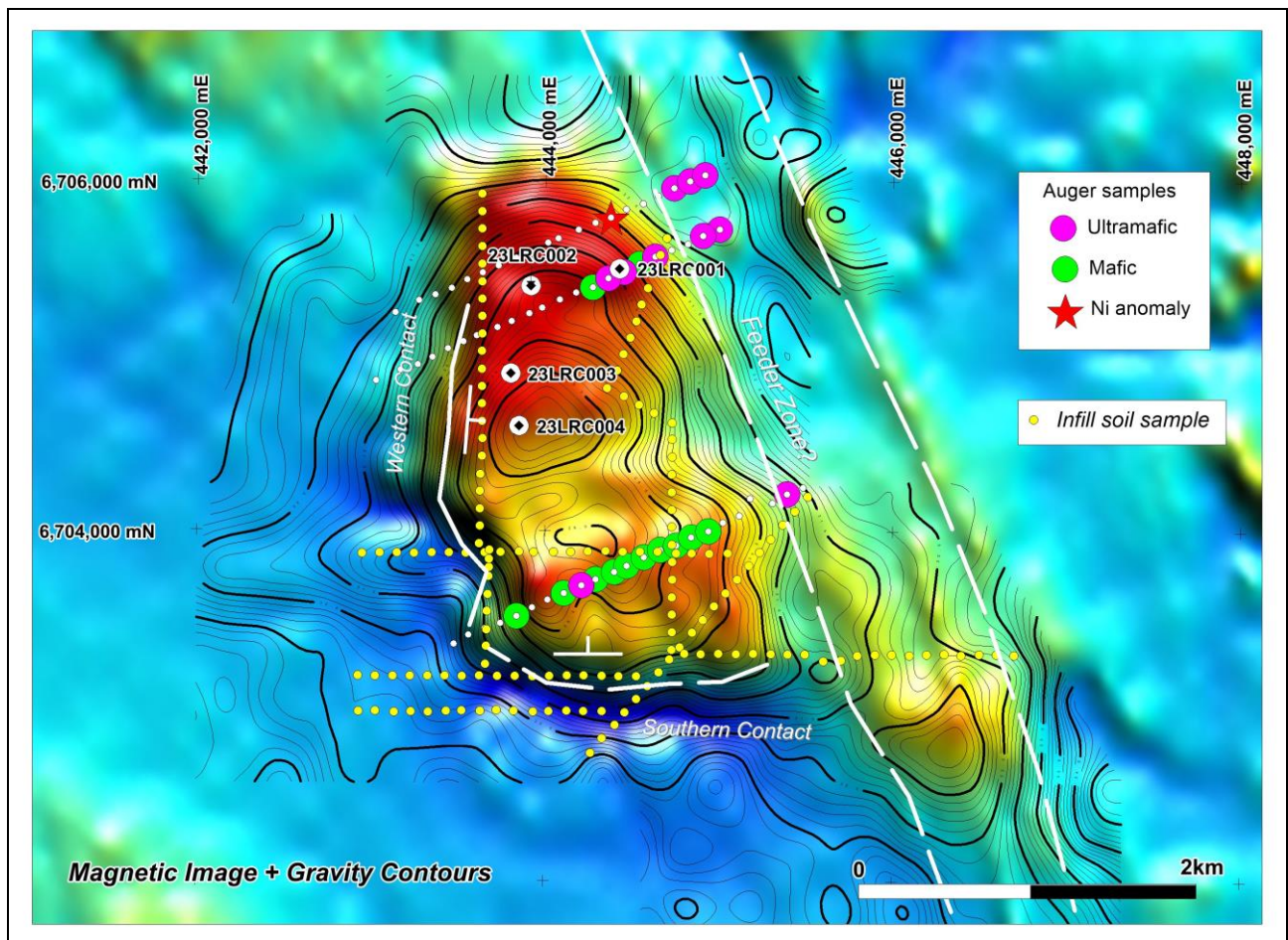
Figure 7: Latham Prospect: detailed magnetic and gravity images showing location of soil samples.
