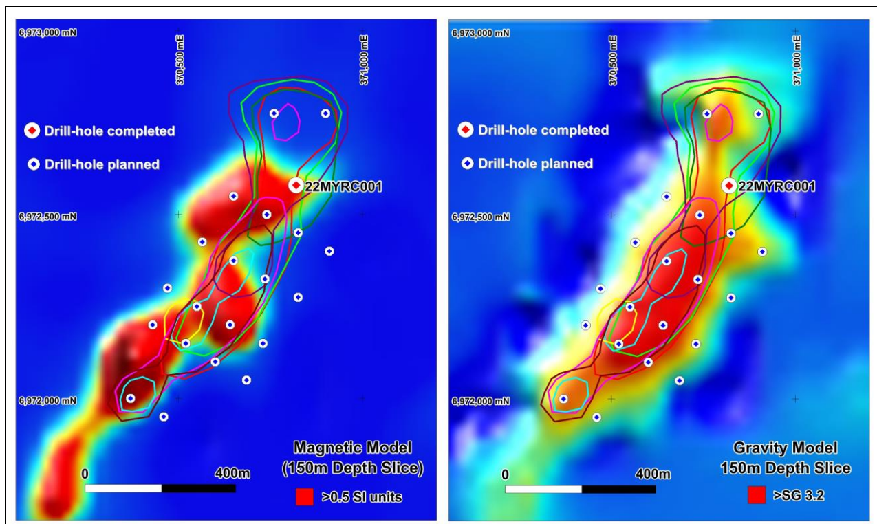
Figure 5: Shows the planned drill-holes with respect to both the magnetic and gravity models. The areas shown in red are both strongly magnetic (magnetic susceptibility >0.5 SI units) and have high density (average SGs >3.2 ), outlining the potential magnetite (Fe) target.
