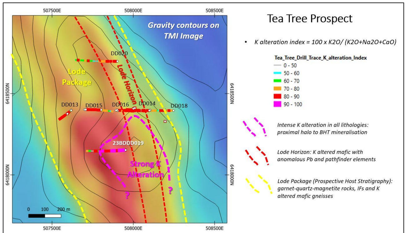
Figure 3: Tea Tree Prospect showing outline of prospective host rocks, lode horizon and potassic alteration as defined by the recent drill-hole geochemistry.
