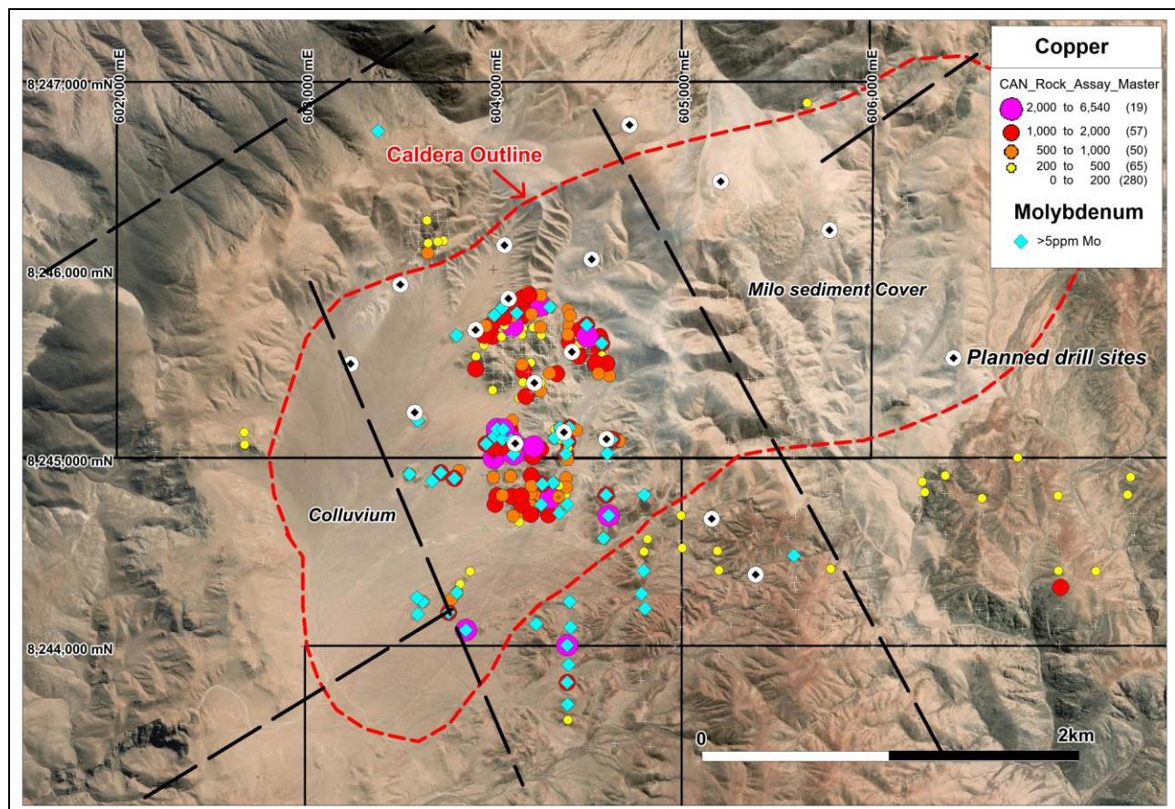
Figure 11: Cangallo Porphyry Prospect showing anomalous Cu and Mo values and planned drill sites.
