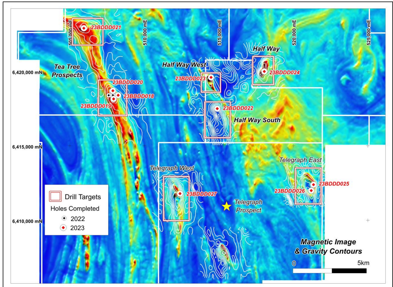
Figure 2: Balladonia Project showing prospect and drill-hole locations on magnetic data.
