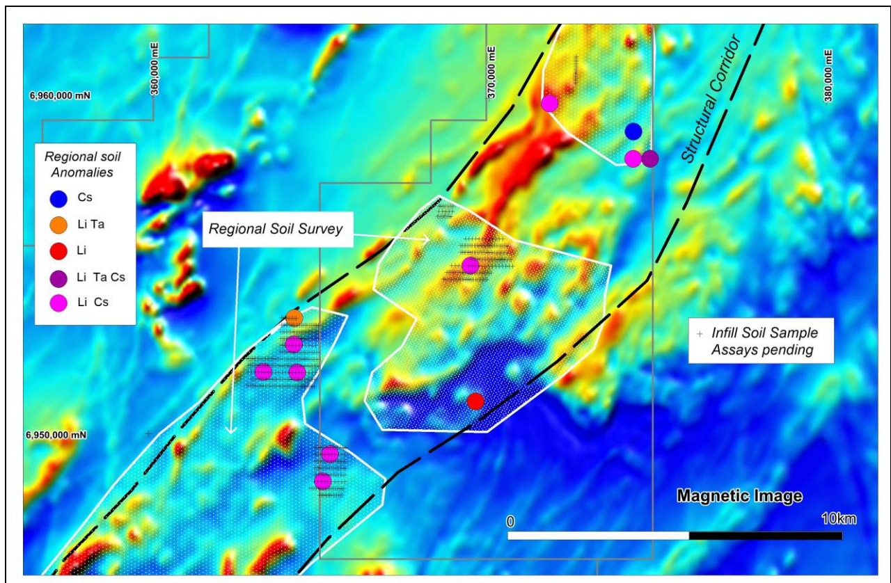
Figure 6: Morrisey – magnetic image showing regional soil anomalies and in-fill soil sample locations.
