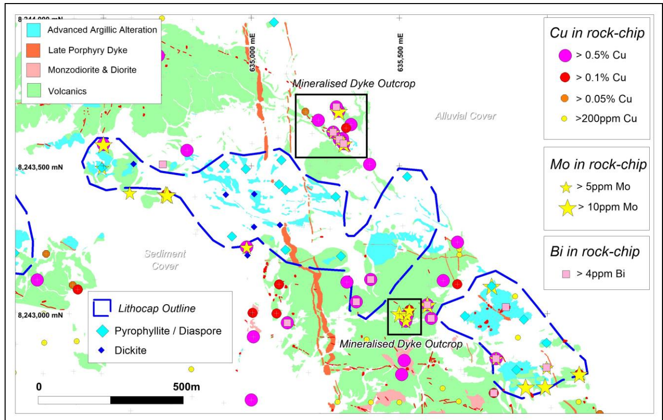
Figure 9: Lantana Prospect geology showing location of mineralised dykes and pathfinder geochemical anomalies marginal to the mapped lithocap.
