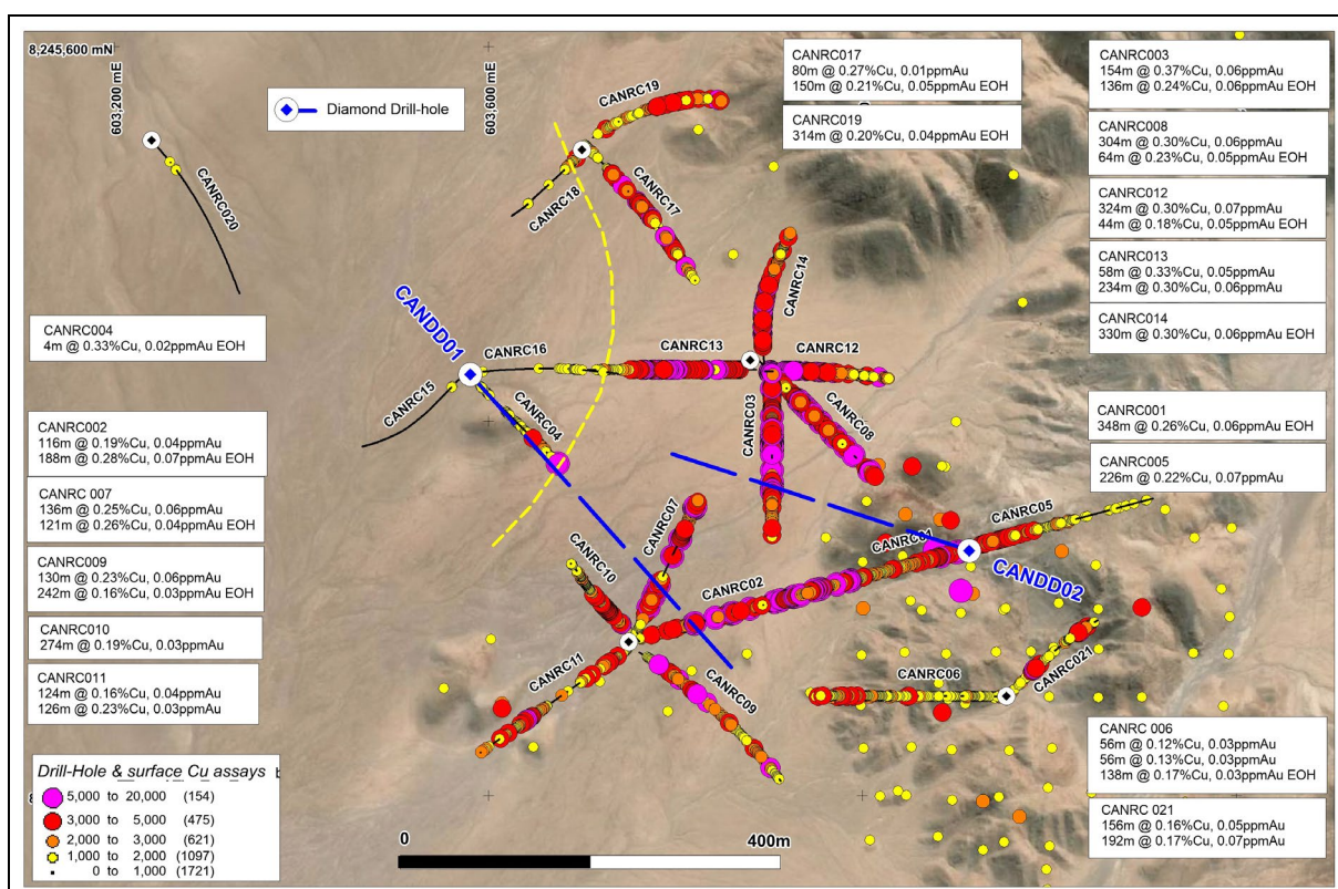
Figure 3: Cangallo Porphyry Copper Prospect showing RC and diamond drill-hole locations and significant intersections.
