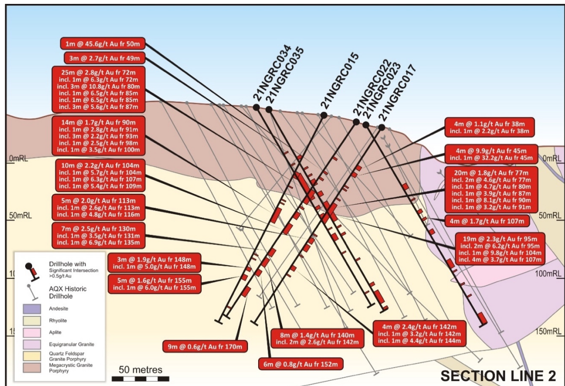
Figure 3 Cross Section Line 2: Phase 1 RC drill locations with significant gold assay intercepts (>0.5g/t Au) (red bars) from recently completed RC holes - 21NGRC015, 21NGRC017, 21NGRC022, 21NGRC023, 21NGRC034 & 21NGRC035. Section also includes previous completed diamond and RC phase 1 drilling traces only.
