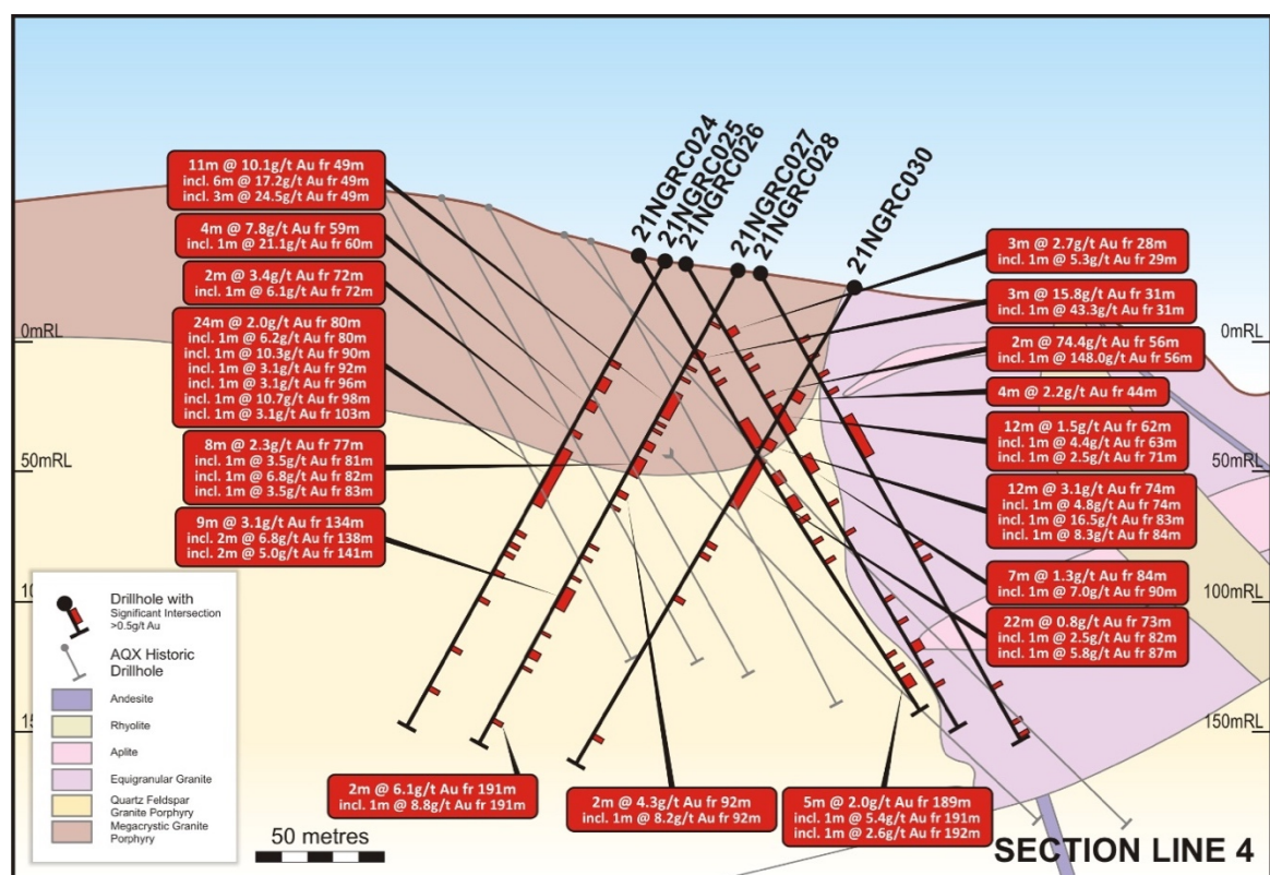
Figure 4 Cross Section Line 4: Phase 1 RC drill locations with significant gold assay intercepts (>0.5g/t Au) (red bars) from recently completed RC holes - 21NGRC024, 21NGRC025, 21NGRC026, 21NGRC027, 21NGRC028, 21NGRC030. Section also includes previous completed diamond and RC phase 1 drilling traces only.
