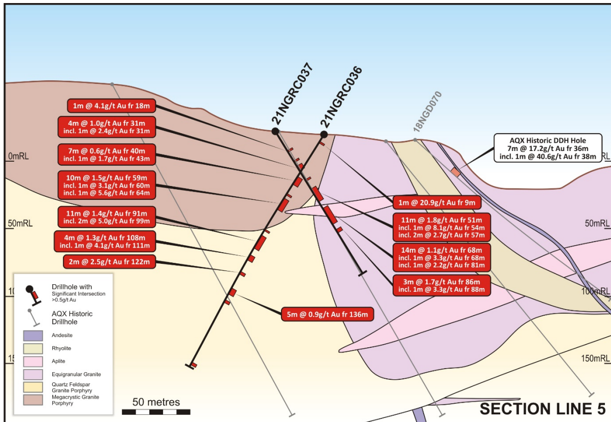
Figure 5 Cross Section Line 5: Phase 1 RC drill locations with significant gold assay intercepts (>0.5g/t Au) (red bars) from recently completed RC holes - 21NGRC036 & 21NGRC037. Section also includes completed diamond and previously reported RC phase 1 drilling Au assay intercepts (>0.5g/t Au)) (black bars)
