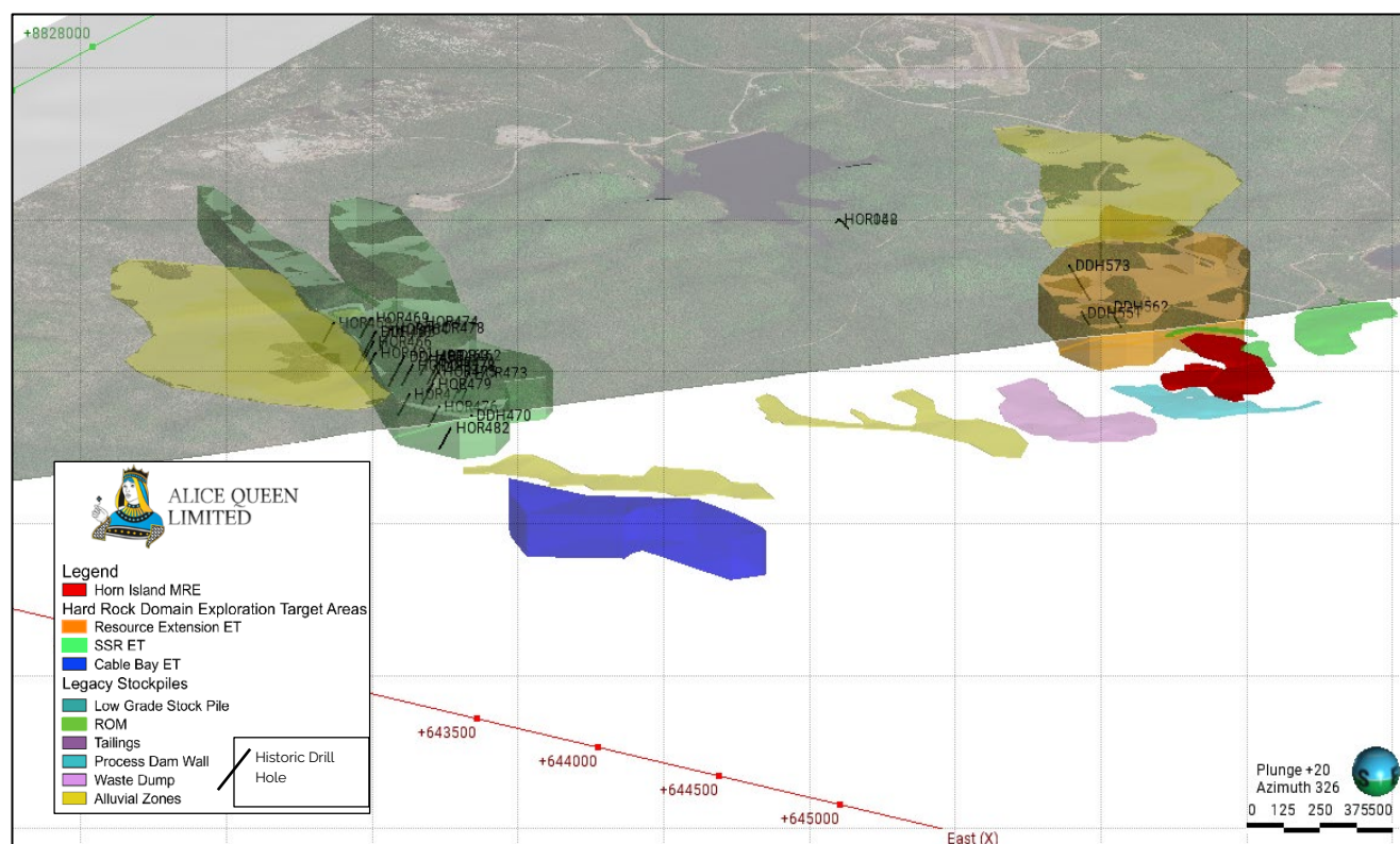
Figure 2: 3D sectional view of exploration target areas with Historic drill hole traces
