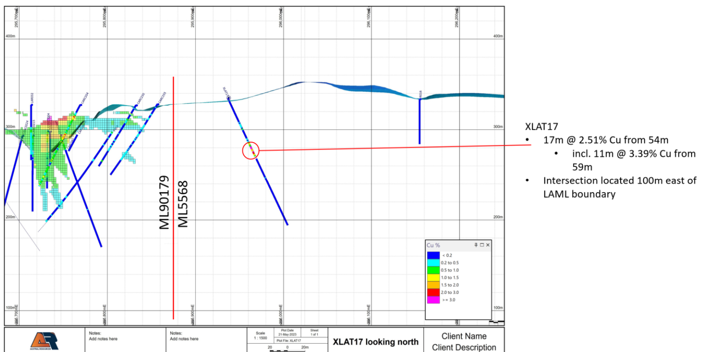
Figure 2. Cross section XLAT-17 Lady Annie / Lady Loretta historical drilling.
