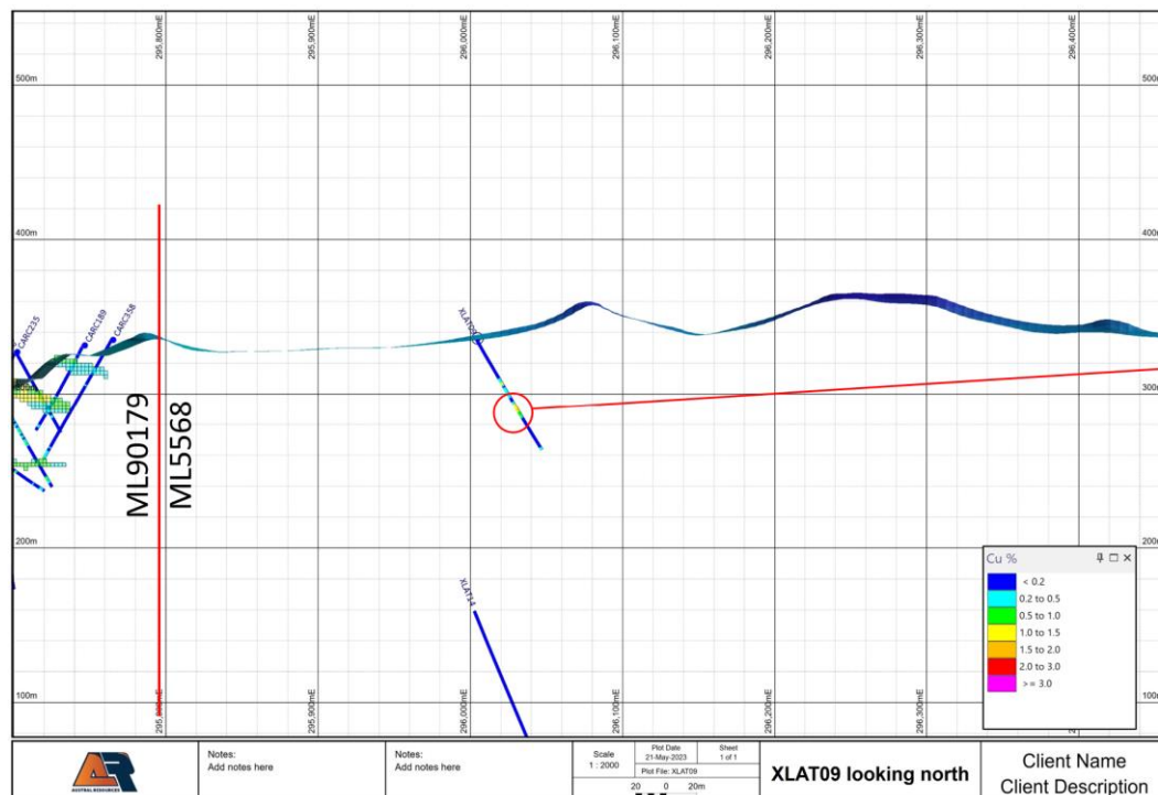
Figure 3. Cross section XLAT-09 Lady Annie / Lady Loretta historical drilling.
