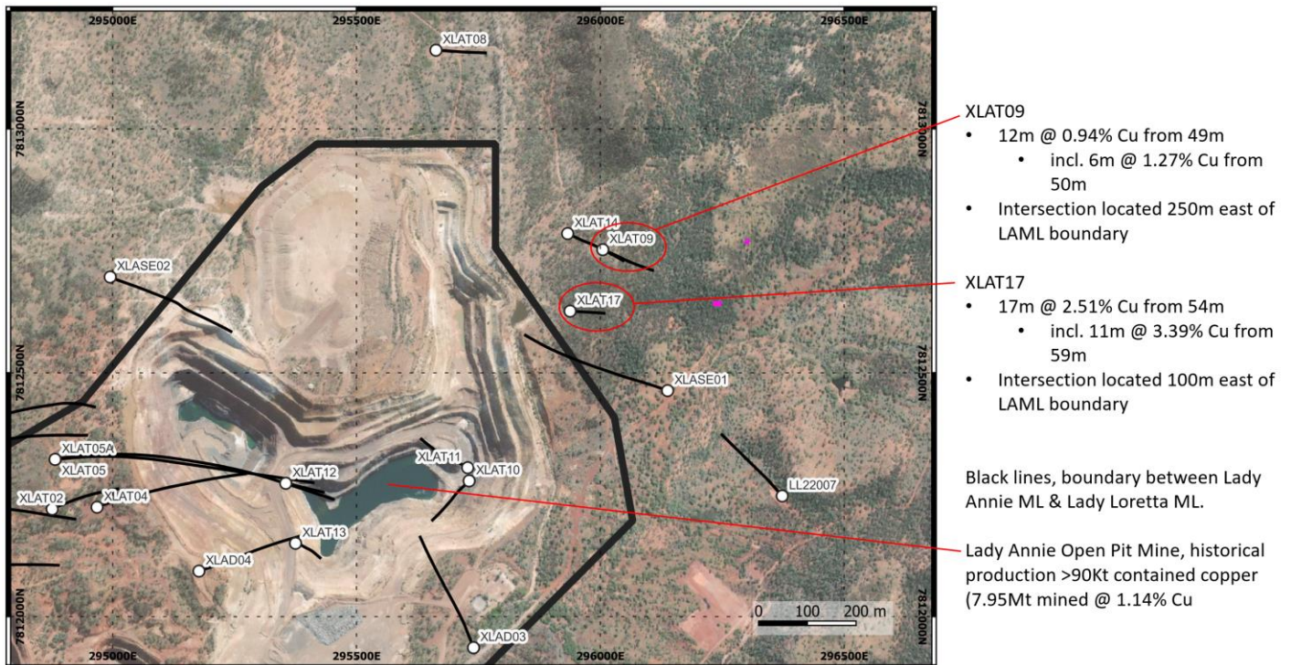
Figure 1. Plan View Lady Annie, Lady Loretta mining lease boundary and drilling traces.
