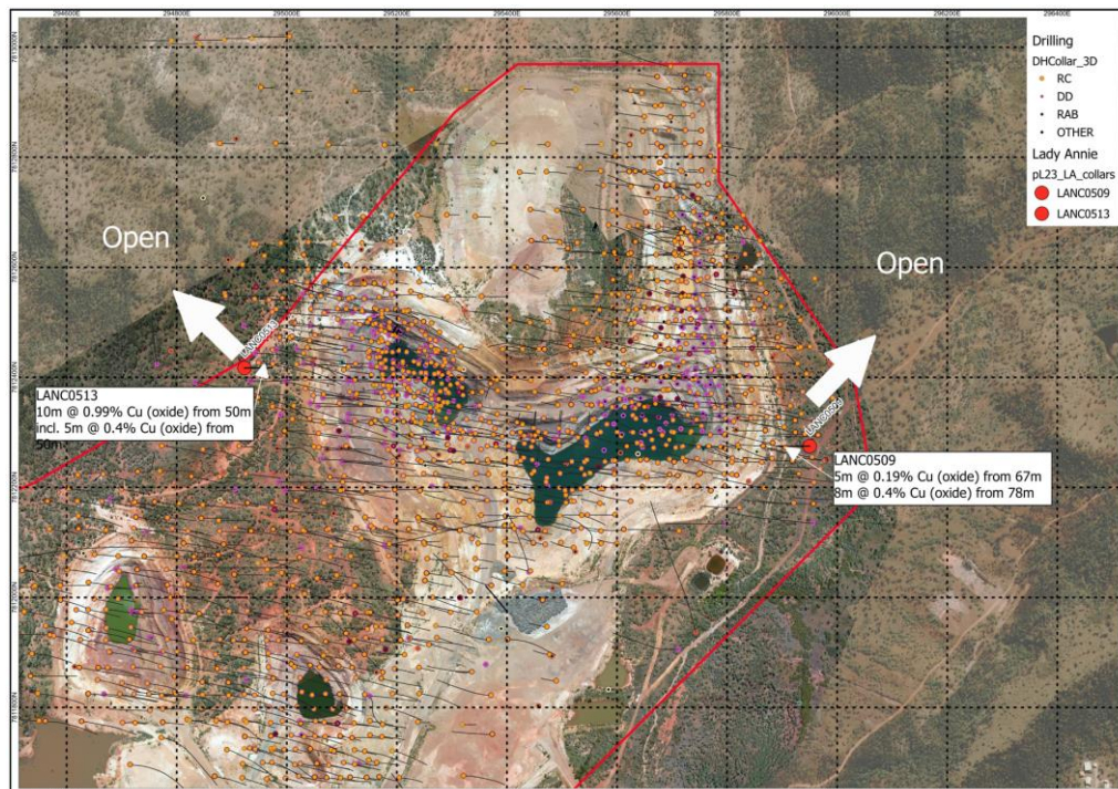
Figure 7. Lady Annie Plan view, location of LANC0513 & LANC0509 and prior drilling.
