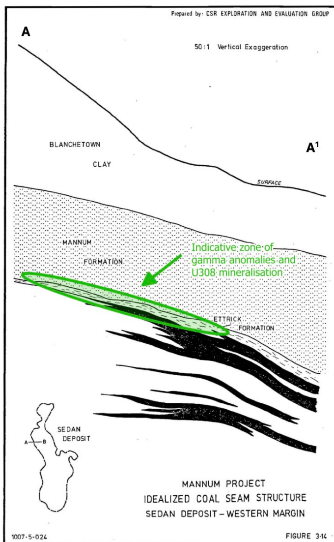
Figure 6 — Western flank zone of interest, through A-A¹, shown with 50:1 vertical Exaggeration. Modified from Open File Envelope ENV03345 pg1759.
