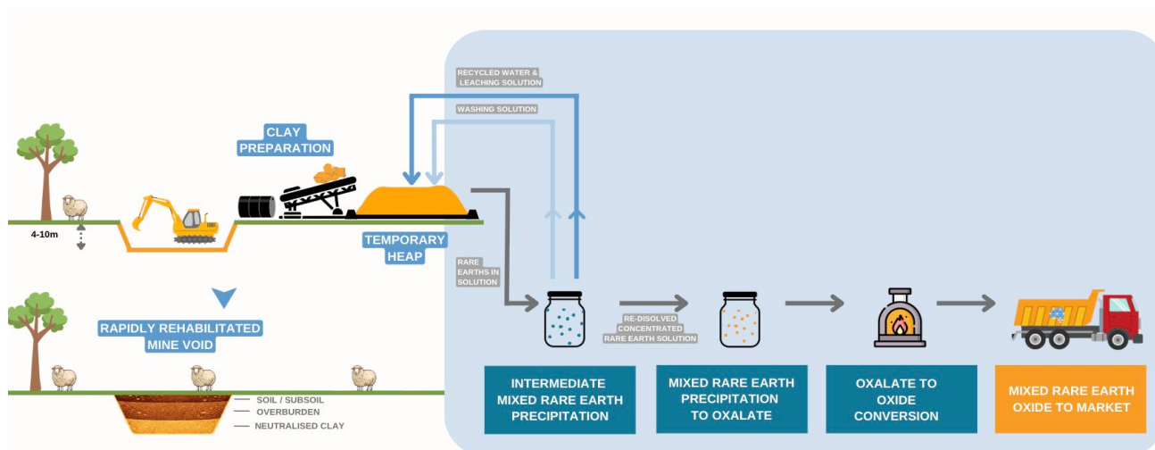
Figure 2 — Koppamurra Conceptual Project Flowsheet showing the five-stage flowsheet from clay preparation through to Mixed Rare Earth Oxide to market.
