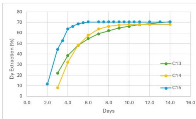
Figure 3 — Dy extraction over time; C15 at double flow rate compared with C13 (50% \text{MgSO}_4 ) & C14 (std conditions).
