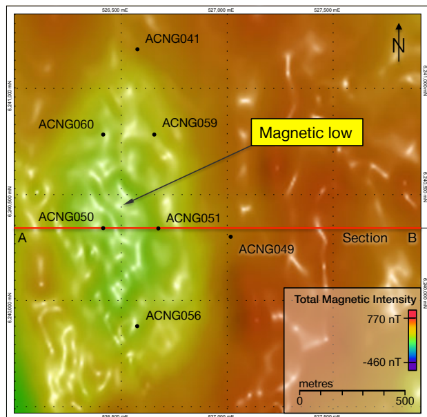
Figure 3a - Magnetic low anomaly (cross section AB)
