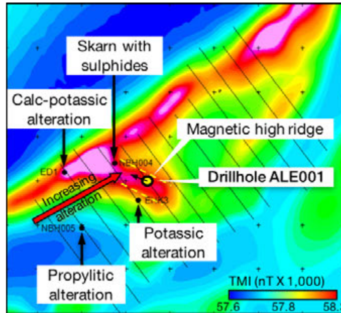
Magnetic survey
