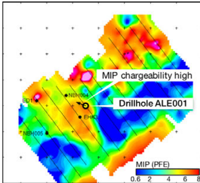
Magnetic induced polarisation (MIP) survey (world first)
