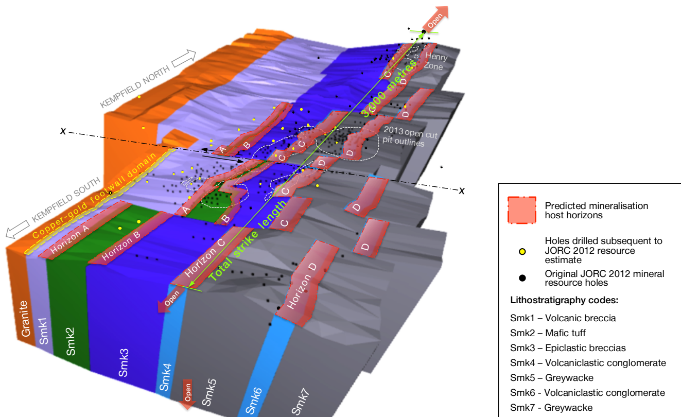
Figure 2 – Illustrating approximate locations of mineralisation host horizons predicted by the mineralisation and genetic model, that will form the basis of the resource infill drilling programme design. Isometric view, facing North.
