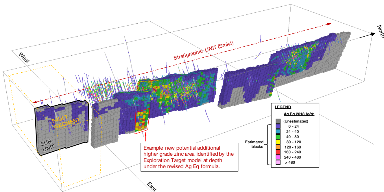
Figure 1 – Example screen shot of the 3D Datamine Unconstrained Estimate model produced by the combined actions outlined in points 1-3. To simplify the view, only one of the seven stratigraphic UNITS is shown – Smk4, with the most southern fault SEGMENT selected by the orange rectangle, to form the example illustrated SUBUNIT.
