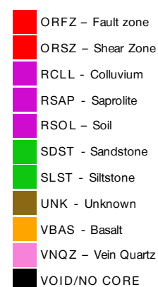
Figure 2 – Stratigraphy legend
