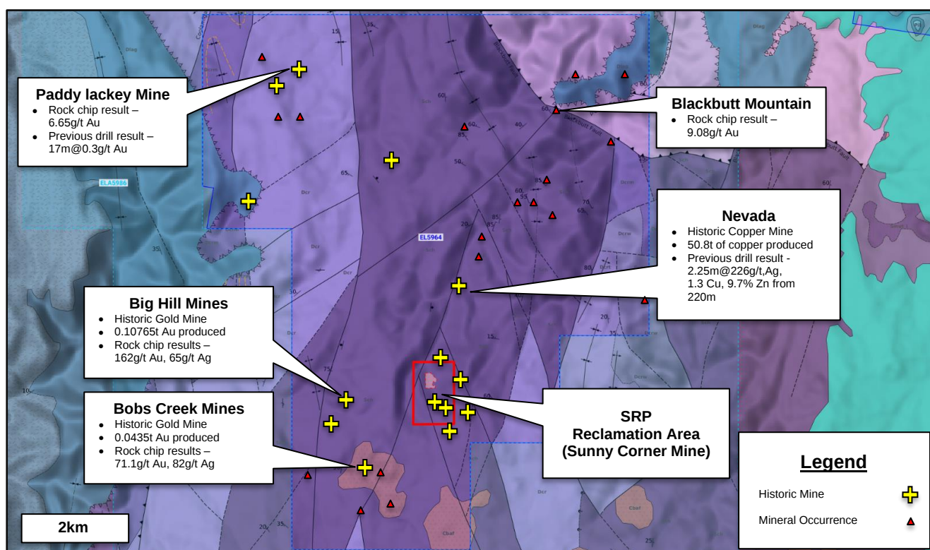
Figure 2 - EL5964 Producing Mines and Mineral Occurrences
