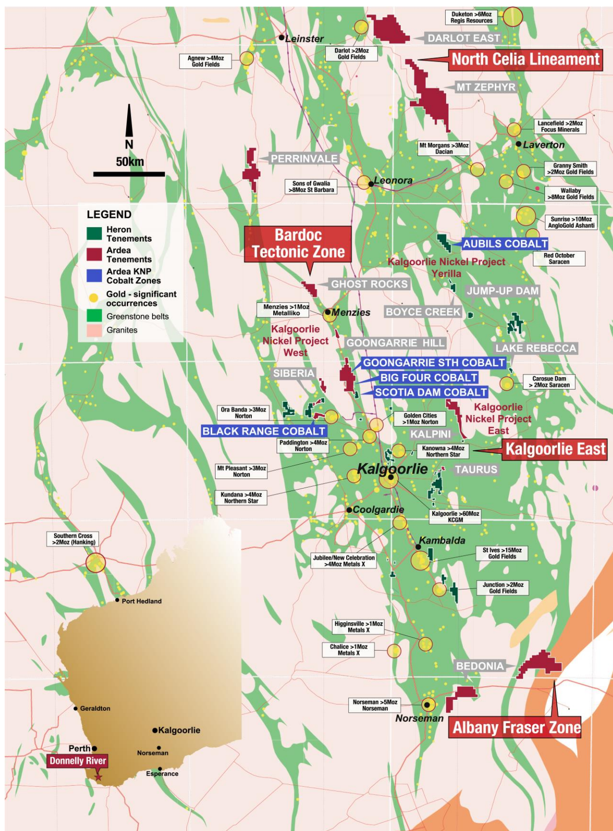
Figure 3 – Ardea WA projects, showing the Goongarrie South, Big Four, Scotia Dam, Black Range and Aubils Cobalt Zones.
