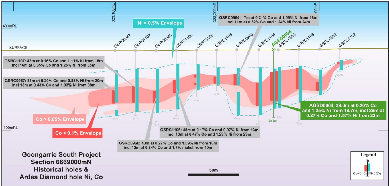
Figure 5 – The 6669000mN sections, showing drill hole AGSD0004 with historic holes and mineralisation distributions. The 0.05 % and 0.10 % cobalt grade shells were generated for, and are consistent with, those shown both in the June 2017 resource upgrade and in plan view in Figure 3. Nickel-based intervals (at 0.5 % cut-off) define an envelope encasing cobalt mineralisation.
