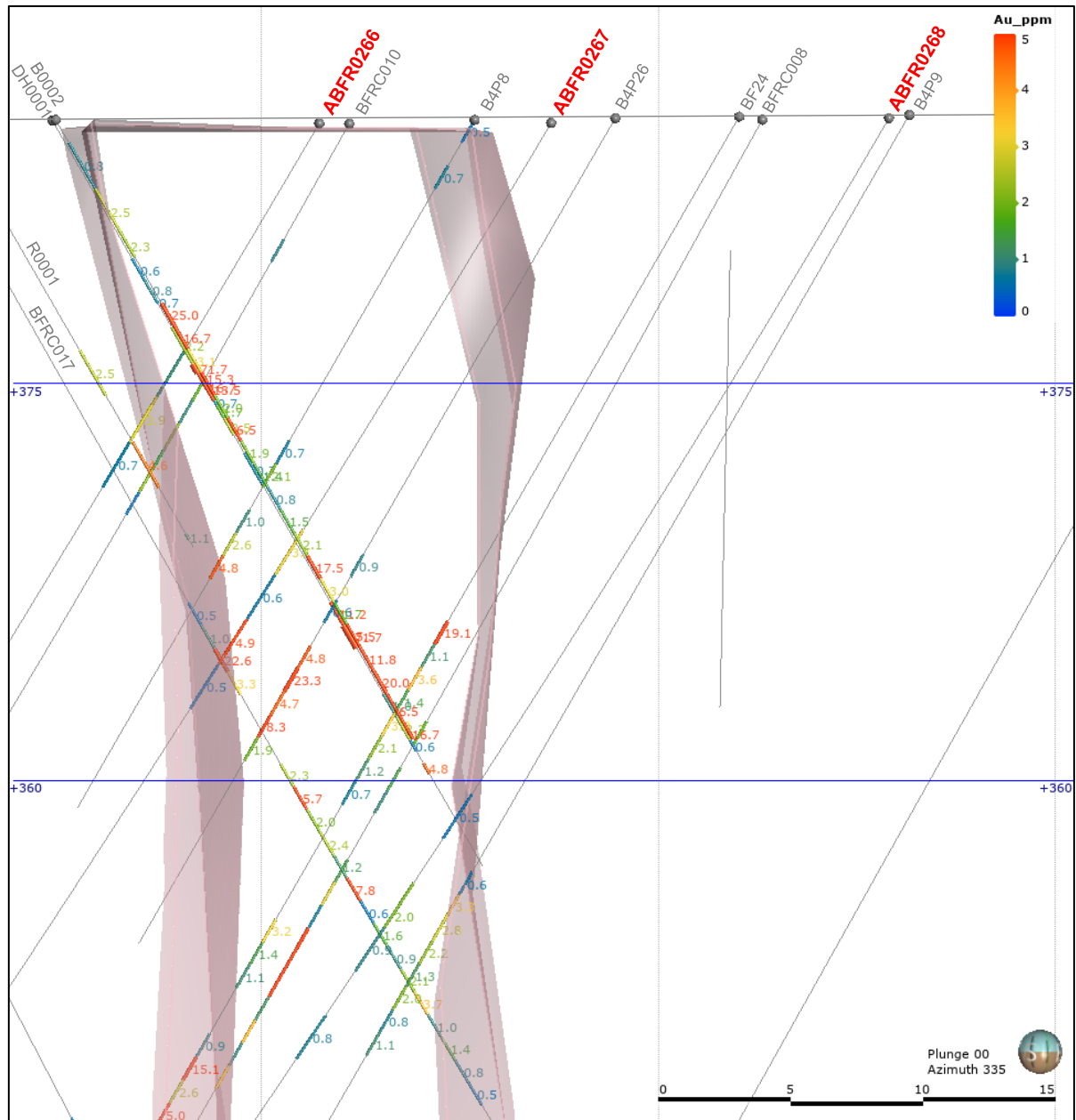
Figure 2 – Cross section 6663360mN +/- 5 m of the Big Four Gold deposit. Twinned pairs are as follows: ABFR0266 & BFR010, ABFR0267 & B4026, ABFR0268 & B4P9. The Big Four Gold porphyry is shown in transparent pink. Looking towards 335°. Projection: GDA94 MGA Zone 51.
