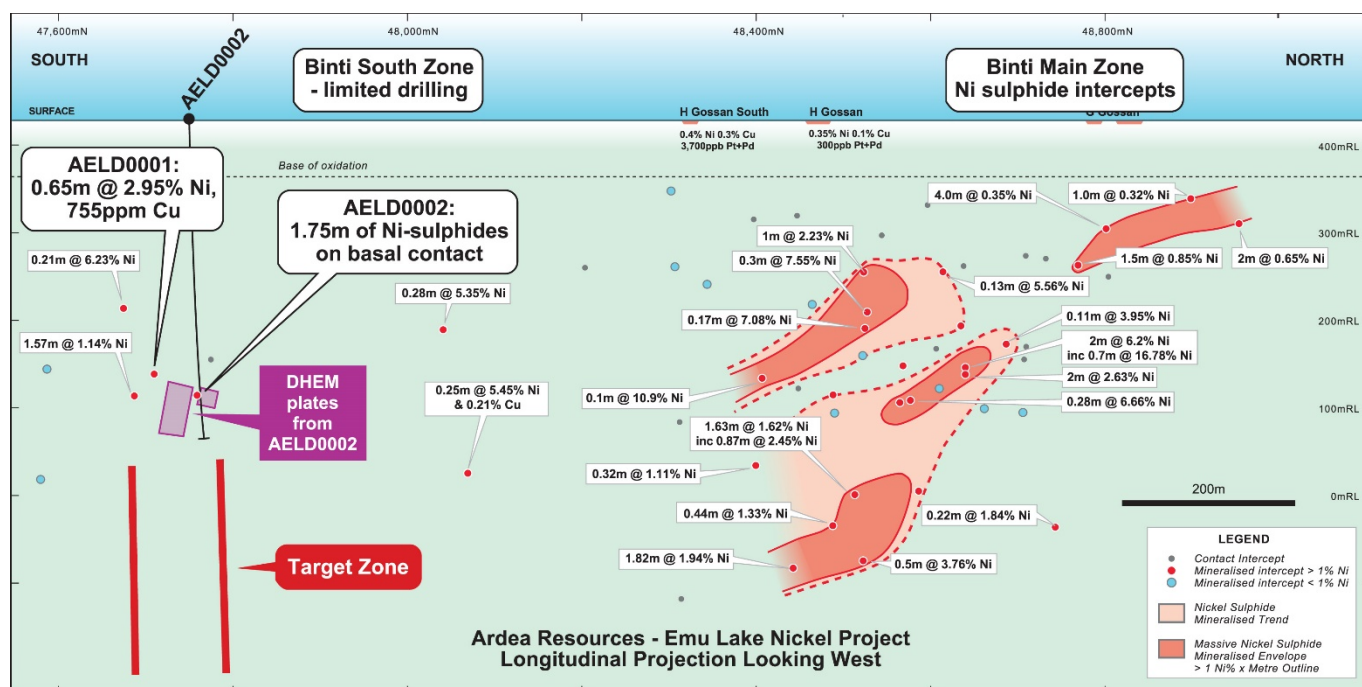
Figure 5: Emu Lake long section looking west showing new DHEM conductors generated from surveying recently completed drill hole, AELD0002.
