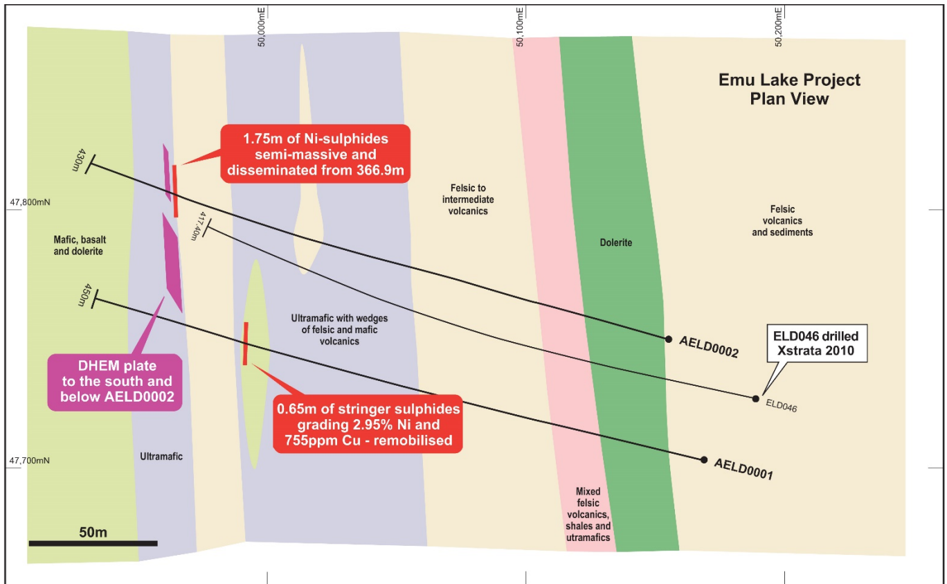
Figure 3: Emu Lake prospect in plan view, showing recent drilling and DHEM plates, local Binti grid.
