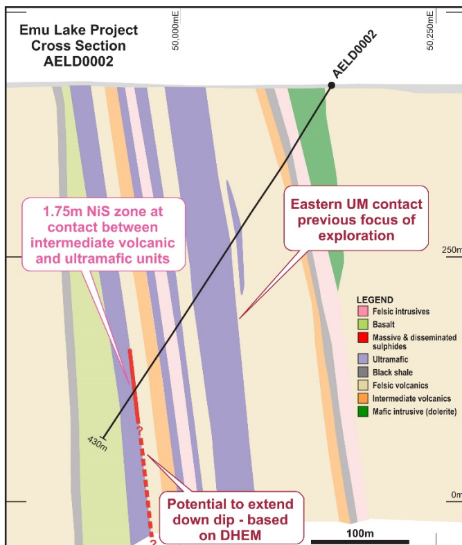
Figure 4: Emu Lake cross section looking north showing trace of drill hole AELD0002 and interpreted geology with new nickel sulphide zone on the western upper ultramafic unit. DHEM modelled plates for AELD0002 are also shown with the larger plate being slightly south of the hole.
