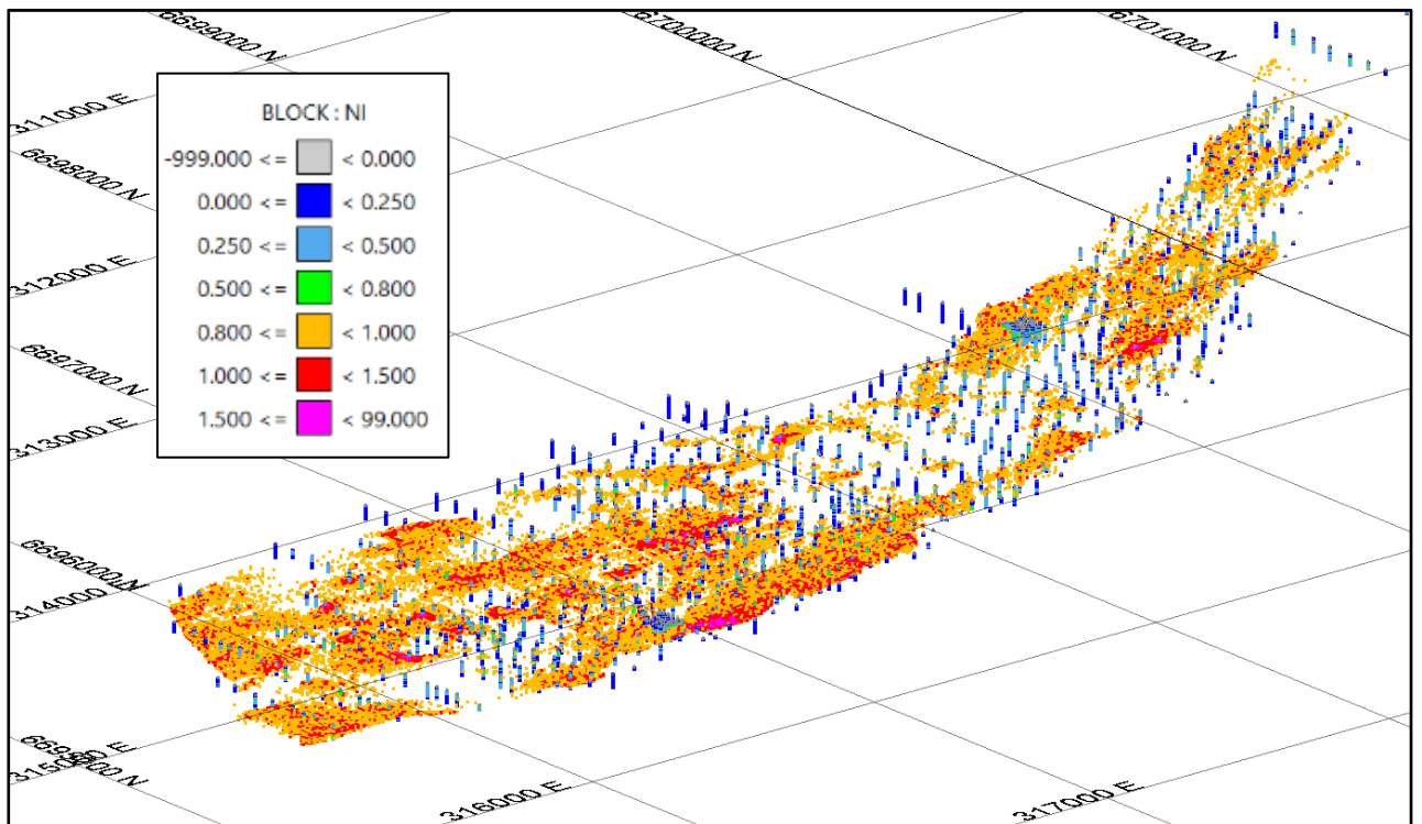
3D view looking -20^\circ towards azimuth of 310^\circ showing continuity of MRE block model blocks \geq 0.8\% Ni versus drillhole traces colour coded by Ni % (same as block legend)
