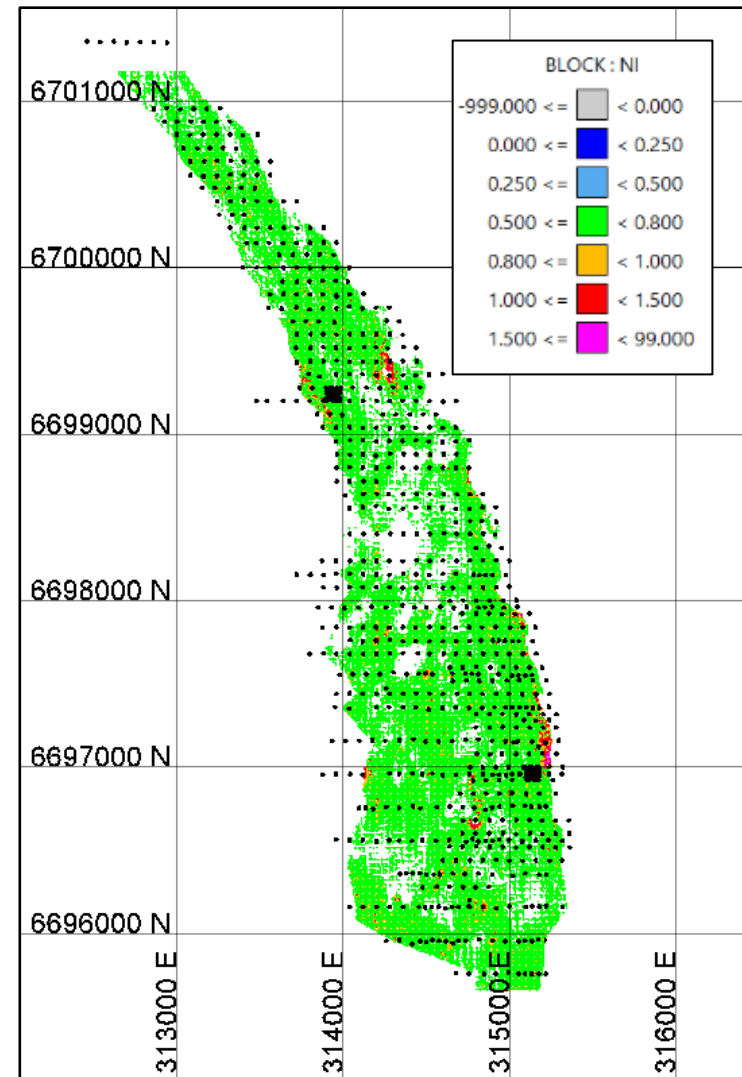
Figure 6-2: Plan view of MRE block model nickel grades of top exposure of Clay Upper material types \geq 0.5\% Ni
