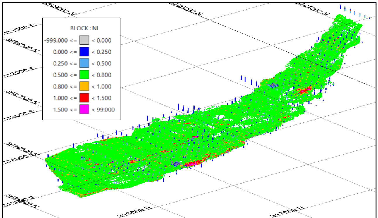
3D view looking -20^\circ towards azimuth of 310^\circ showing continuity of MRE block model blocks \geq 0.5\% Ni versus drillhole traces colour coded by Ni % (same as block legend)
