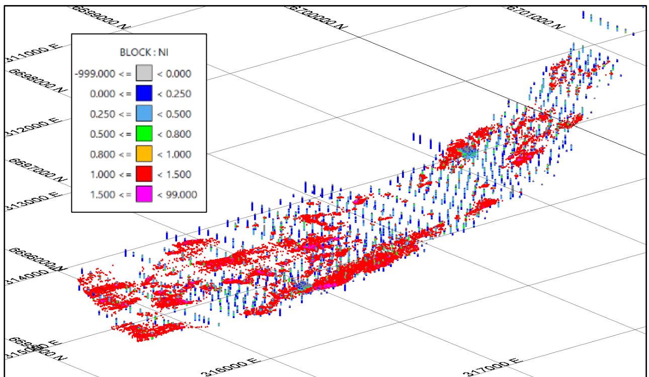
3D view looking -20^\circ towards azimuth of 310^\circ showing continuity of MRE block model blocks \geq 1.0\% Ni versus drillhole traces colour coded by Ni % (same as block legend)
