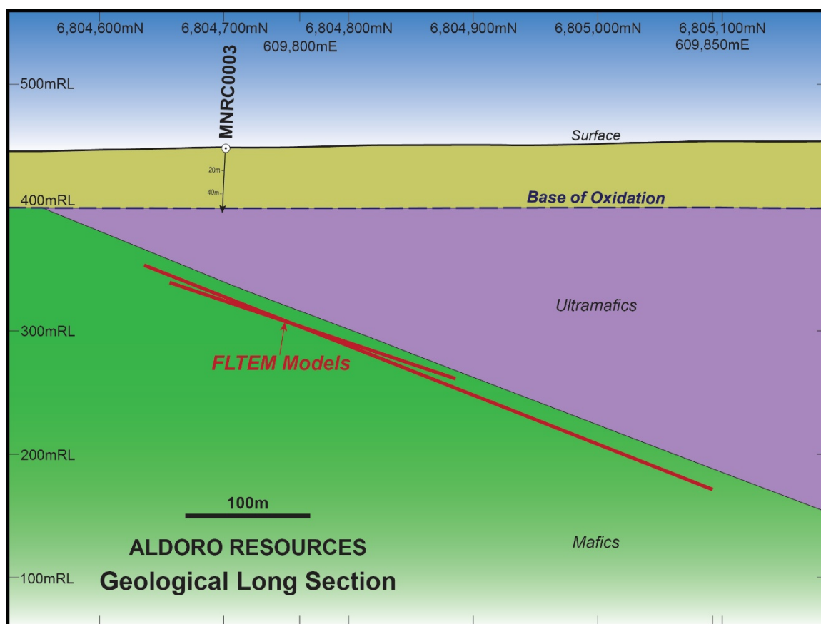
Figure 3. Longitudinal section, looking west north-west, of the VC1 exploration target, showing the favourable geological setting, and the proximity of drillhole MNRC0003, which continues off section to the west.
