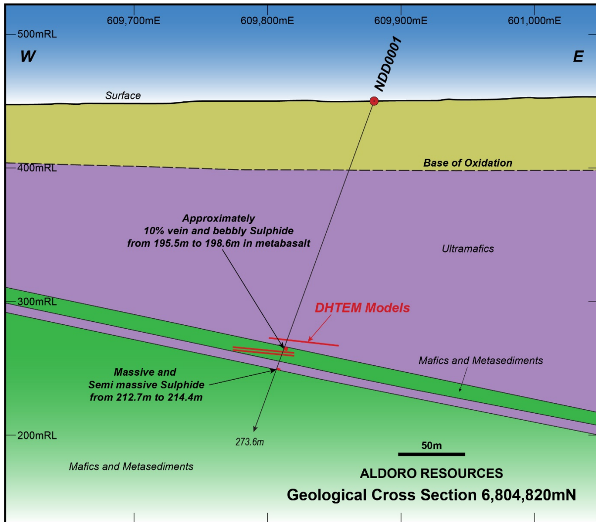
Figure 5. Cross-section of NDD0001 at 6804820m north (MGA50)
