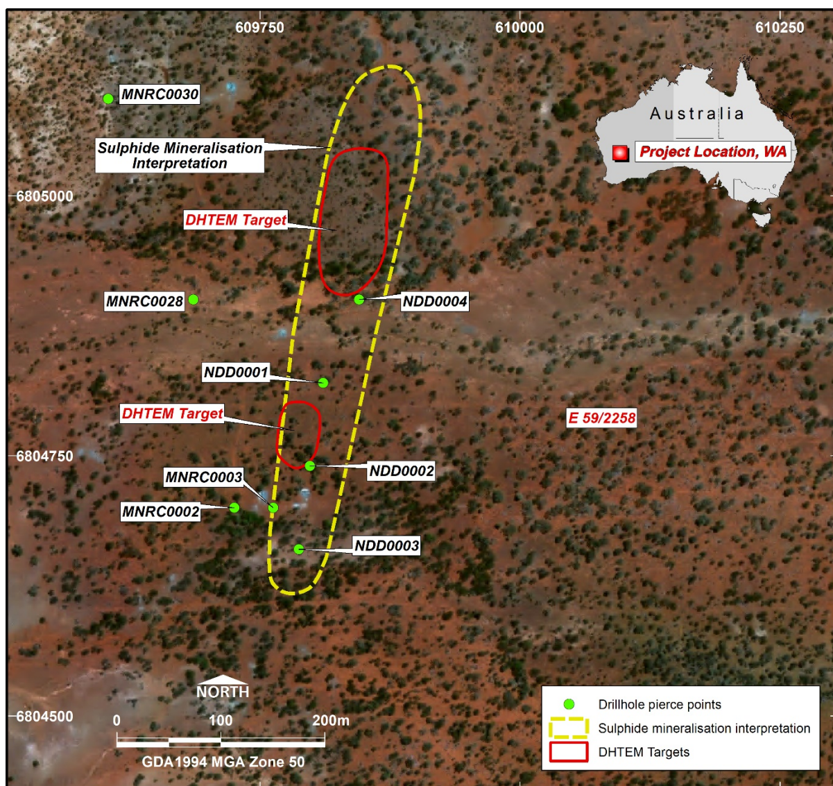
Figure 2. Plan projection showing completed drillhole pierce points of the VC1 target and an evolving interpretation of the magmatic sulphide footprint. DHTeM surveying generated the two high priority off-hole conductors shown in red. DHTeM surveying indicates that the anomaly is strengthening north of NDD0004.
