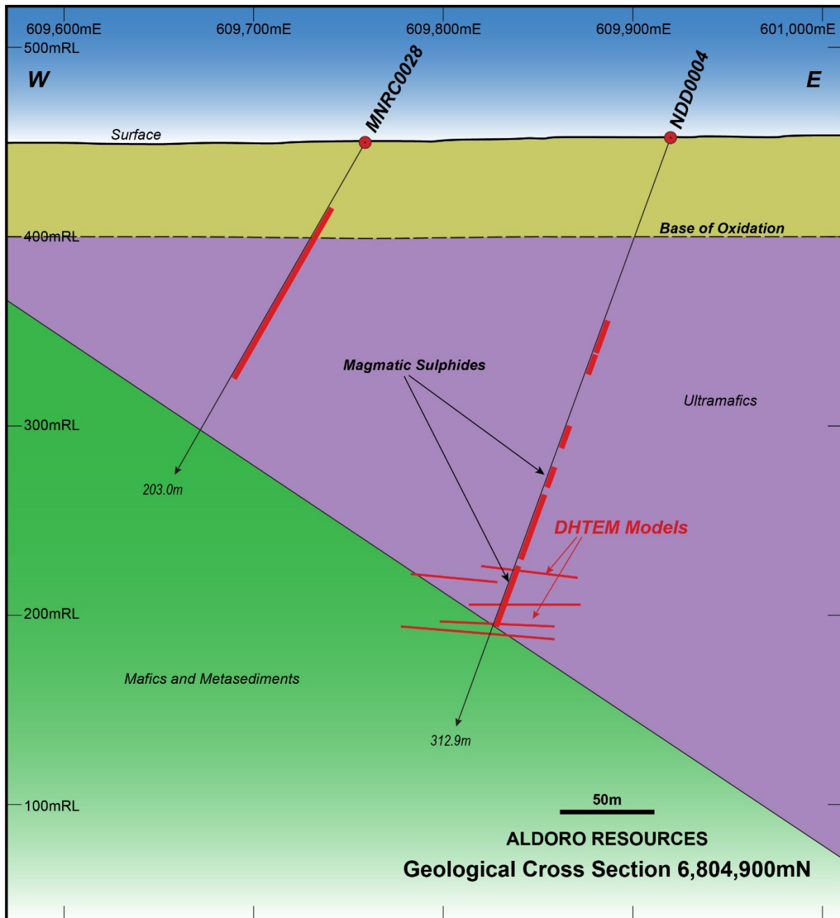
Figure 6. Cross-section of NDD0004 at 6804900m north (MGA50)
