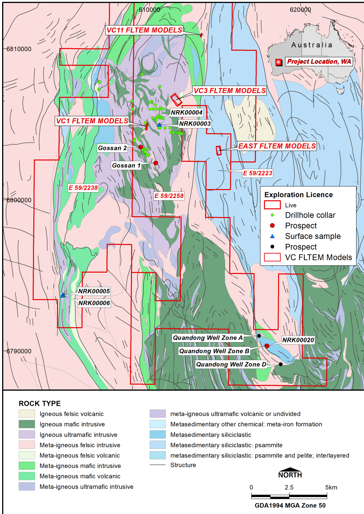
Figure 8. Geological map of the NIC, showing the location of drill ready MLTEM targets and drillhole NDD0001.
