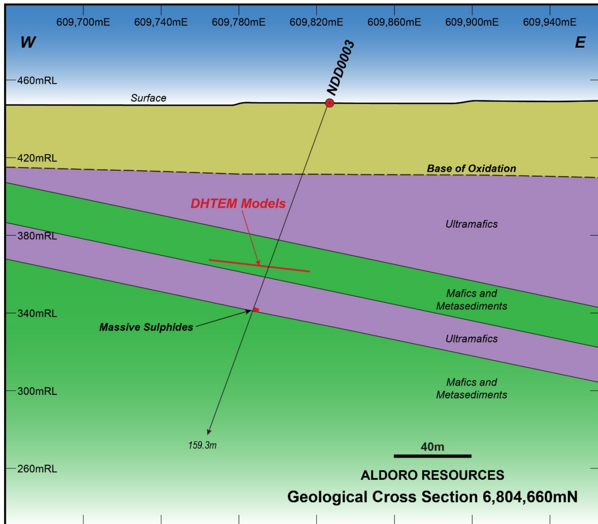
Figure 3. Cross-section of NDD0003 at 6804660m north (MGA50)
