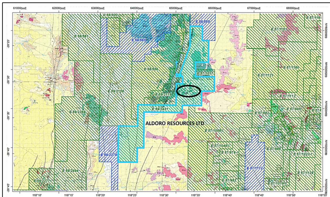
Figure 14. Map showing the location of the LCT pegmatite swarm confirmed by field reconnaissance mapping (circled) at tenement E59/2431.
