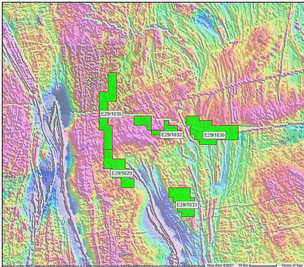
Figure 16. Aldoro's Cathedral's Belt tenements superimposed over a regional aeromagnetic background.
