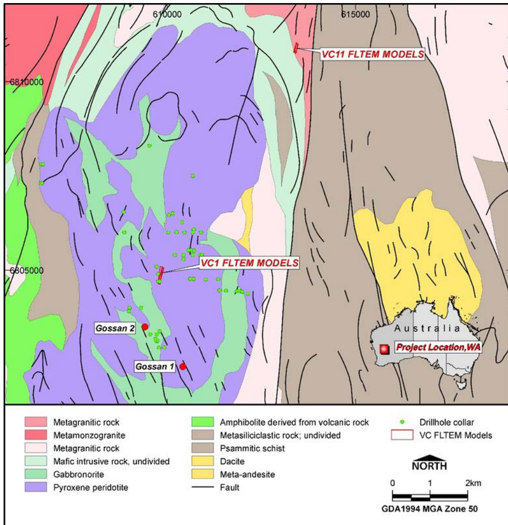
Figure 10. Geological map of the NIC, showing the positions of Gossan 1 and Gossan 2 in relation to the VC1 drill target.
