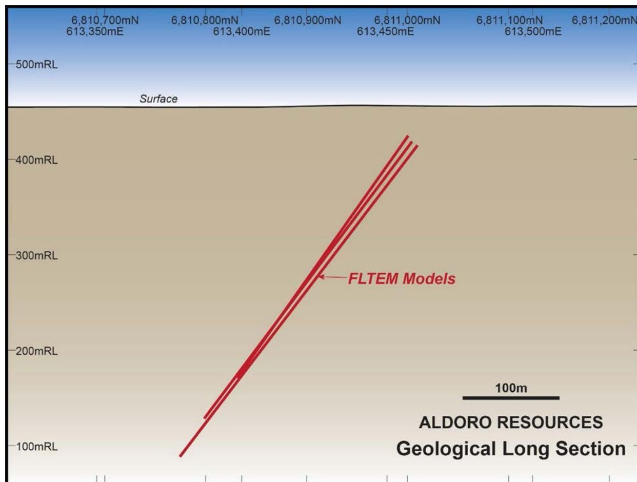
Figure 9. Longitudinal section, looking west north-west, of the VC11 exploration target which has been interpreted to be available for immediate test drilling.
