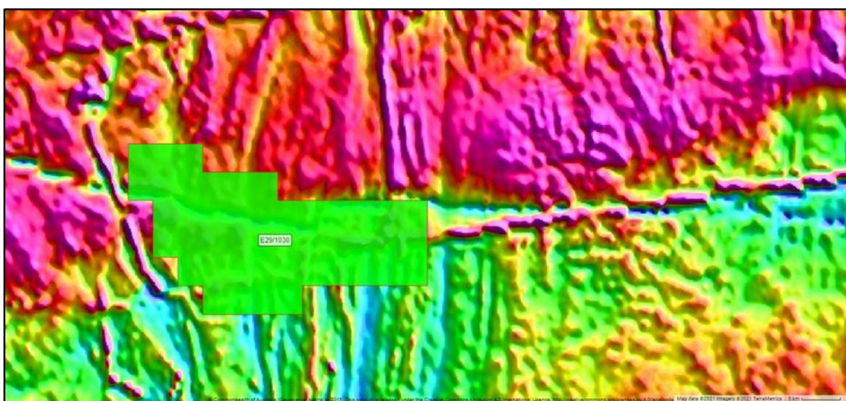
Figure 17. Potential strike extension of E-W nickel-sulphide rich greenstone ultramafic units into E29/1030.
