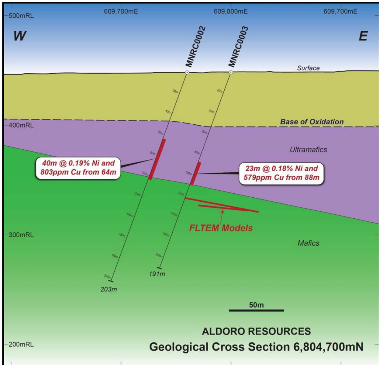
Figure 8. Cross section, looking north, showing proximity of historic drill holes to Aldoro's VC1 bedrock anomaly and drill target
