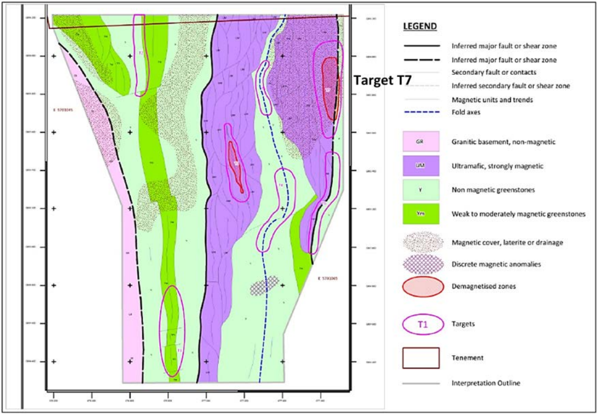
Figure 3. Priority target areas, including the high-priority target T7.
