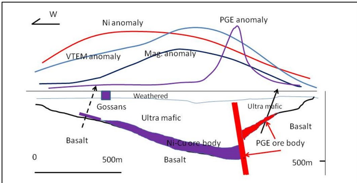
Figure 4: Interpreted geological cross section of Line 5500N
