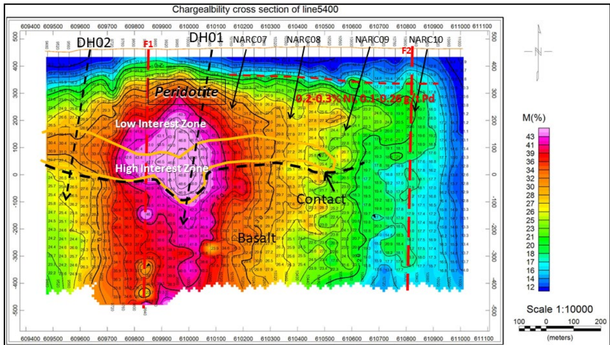
Figure 5: IP Chargeability index cross-section Line 5400 with the High Interest Zone interpreted as a possible zone of massive sulphide along the interpreted basal ultramafic – mafic contact zone. The Low Interest Zone is interpreted as a zone of possible disseminated sulphides. RC drilling by Falconbridge (NARC007-010 -2004) failed to intersect the High Interest Zone at depth, while the margin to the Low Interest Zone reported Ni up to 0.3% and Pd up to 0.26%. Two faults have been interpreted and are highlighted in the resistivity image, Figure 6.
