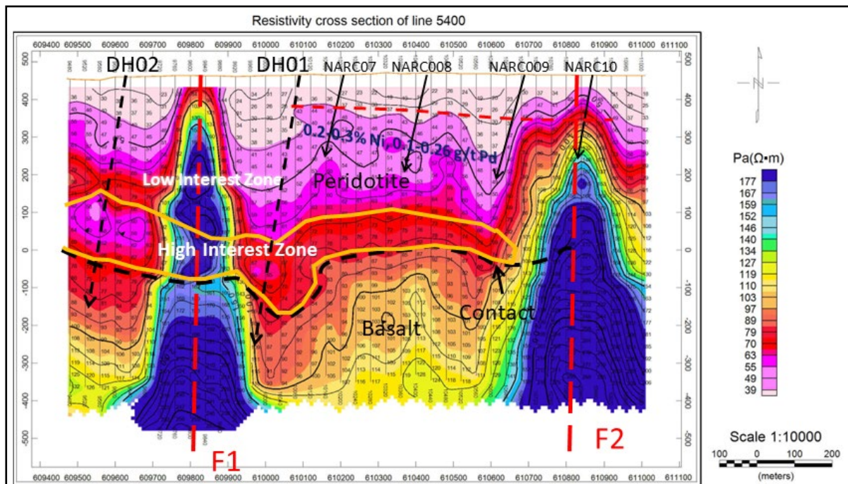
Figure 6: Resistivity profile Line 5400 showing the resistive nature of the faults and highlighting the contrast of the inferred contact between the basal peridotite and basalt and the High Interest Zone interpreted as a possible zone bearing massive sulphide for drill testing (DH01 and DH02).
