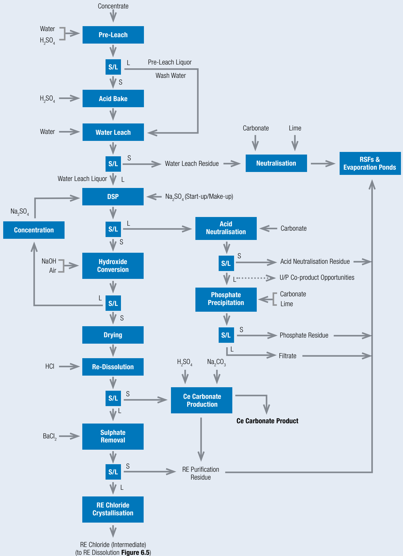
▼ Figure 6.4: RE Extraction Flowsheet
