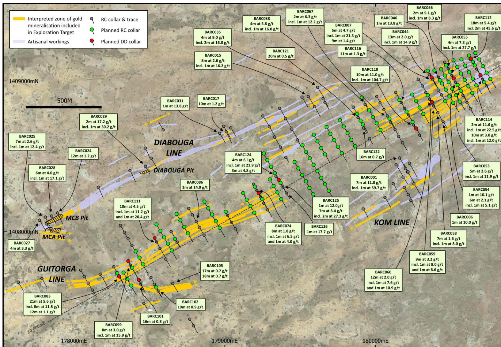
Figure 1. RC drill collars labelled with >10 m x g/t gold intercepts and the interpreted zones of gold mineralisation over a satellite image at Banouassi. The location of the proposed RC holes and diamond holes for the current drilling program are shown in green and red circles respectively.
