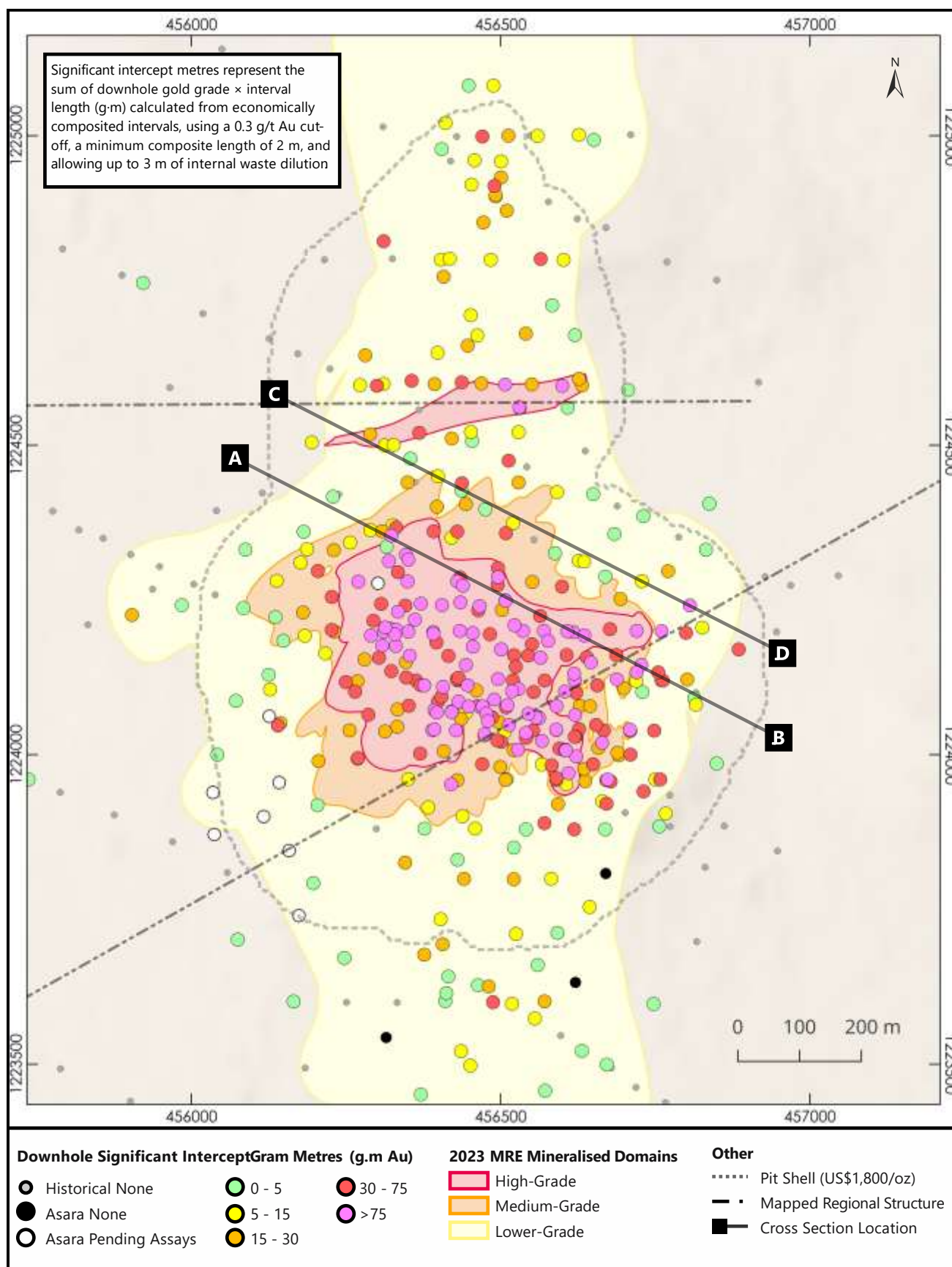
Figure 3: Plan map of the drill collar downhole significant intercepts g.m Au and the location of cross section AB and CD.
