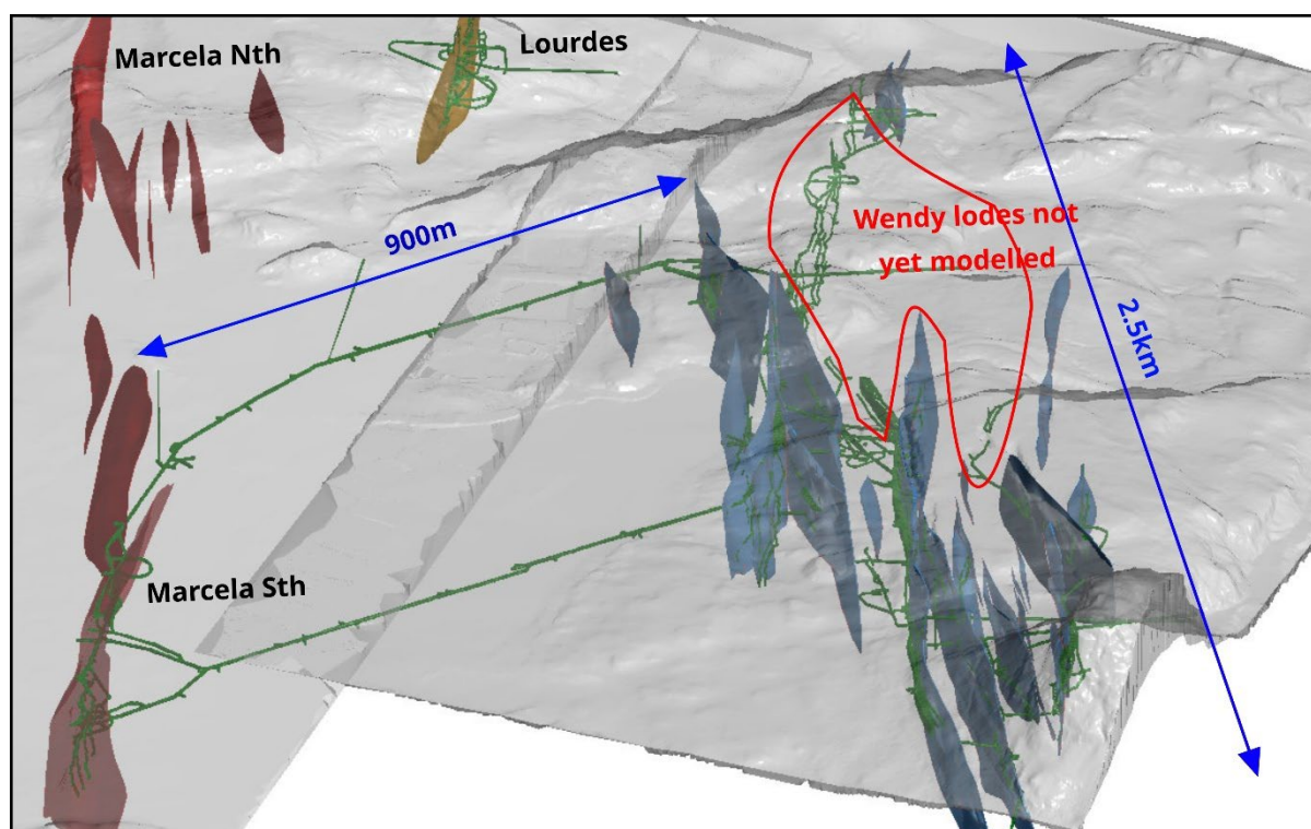
Figure 3. Cerro Bayo Mine Complex (CBMC) showing infrastructure positions linking the Marcela Resource (maroon) and the Cerro Bayo Resource (teal). Wireframes are within current MRE. The historic drill results from the Wendy prospect are still to be modelled and incorporated in a MRE due in early 2025.
