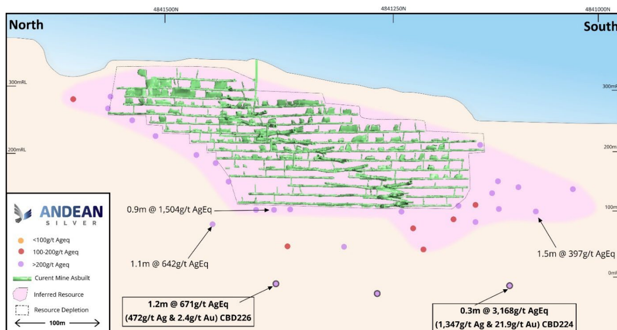
Figure 7. Long Section looking East of Fabiola mine. Latest drilling results in boxes. Refer to Appendix B of this release for latest drilling results and Appendix C for newly reported historical results.
