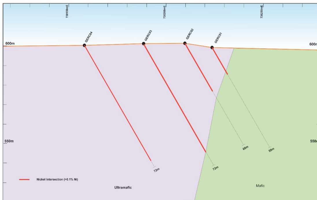
Figure 4: Cross section showing the nickel intersections, 7020595mN.
