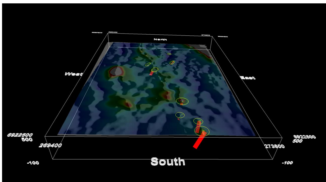
Figure 2: The modelled EM conductor plates at Mary Springs.
