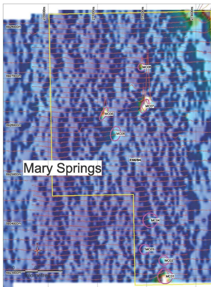
Figure 1: VTEM Imagery (CH48BZ with stacked profiles and targets circled).
