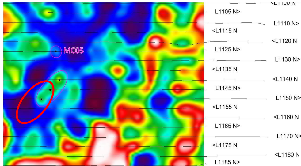
Figure 1: A weakly conductive feature interpreted from VTEM data, south of anomaly MC05
