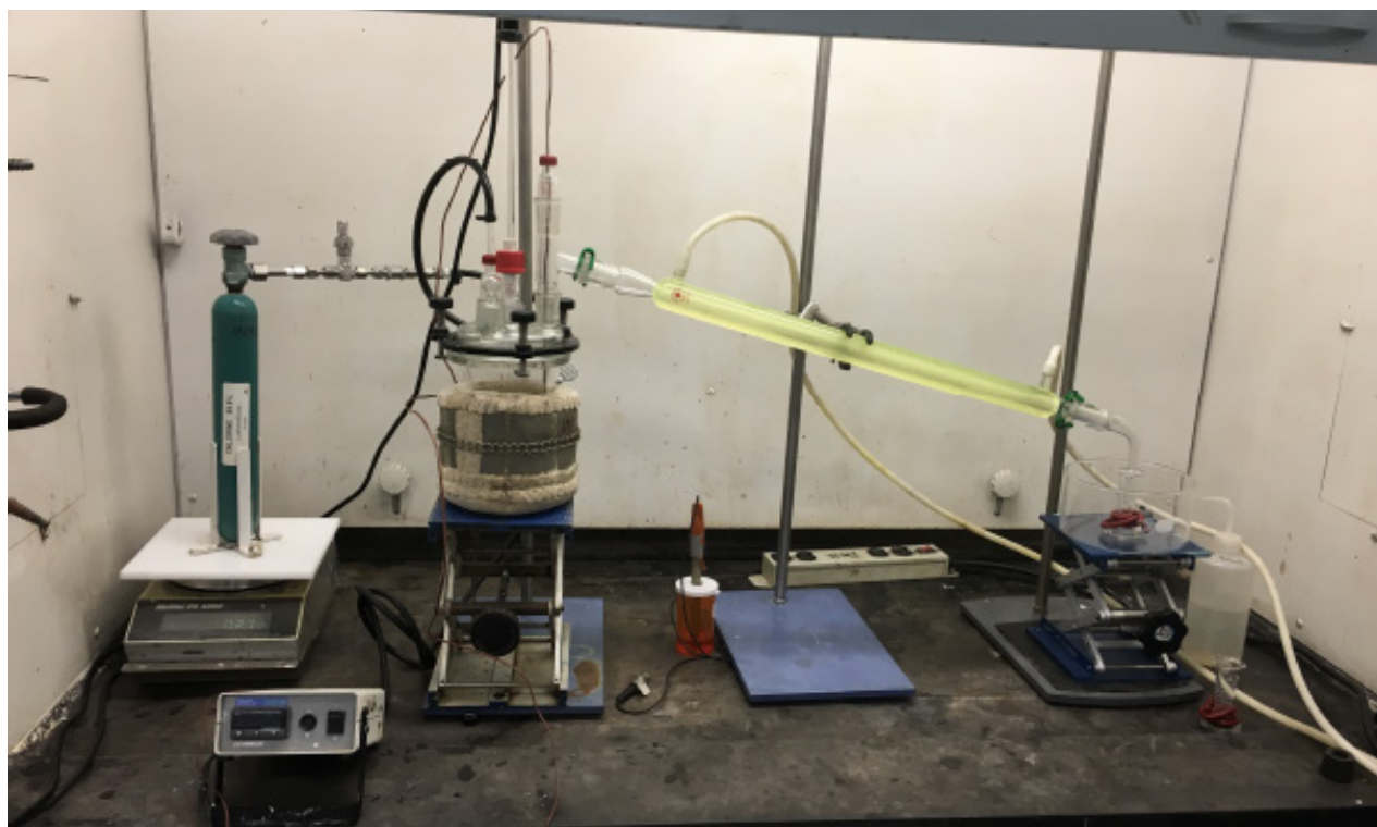
Photo 1: Bromine recovery apparatus
