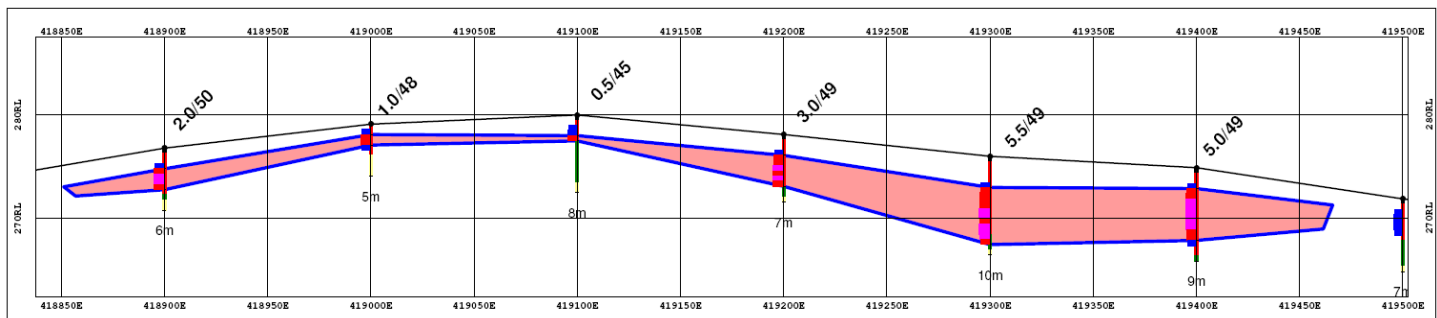
Figure 5: 6,534,400N - typical section through North Bindoon property. Legend – 3.0/49 = 3 metres at 49% \text{Al}_2\text{O}_3 , blue histogram >40% \text{Al}_2\text{O}_3 , red histogram >45% \text{Al}_2\text{O}_3 and magenta histogram >50% \text{Al}_2\text{O}_3 .
