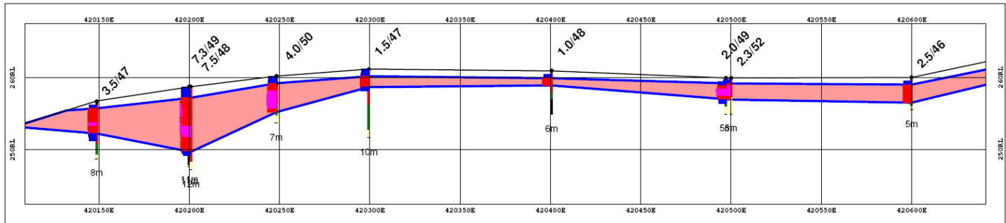
Figure 4: 6,530,400N Section through the proposed Stage, Hares Hill. Legend – 4.0/50 = 4 metres at 50% \text{Al}_2\text{O}_3 , blue histogram >40% \text{Al}_2\text{O}_3 , red histogram >45% \text{Al}_2\text{O}_3 and magenta histogram >50% \text{Al}_2\text{O}_3
