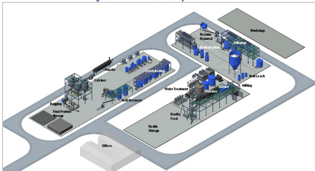
Figure 8 – HPA Plant General Layout and 3D View
