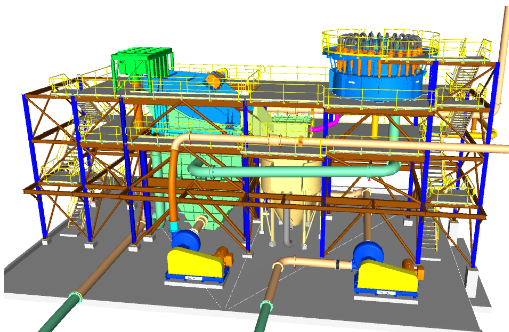
Figure 16 – ROM screen and tails cyclones
