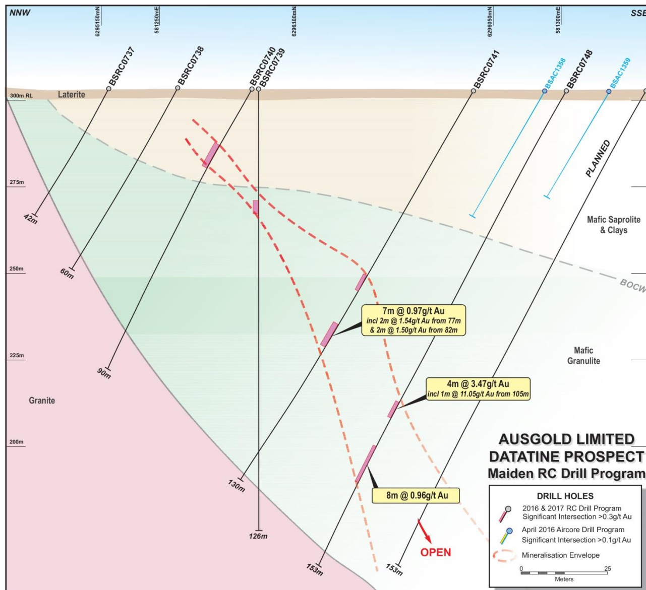
Figure 1. Datatine prospect cross-section showing drill holes, interpreted geology and mineralisation – see Figure 4 for location.
