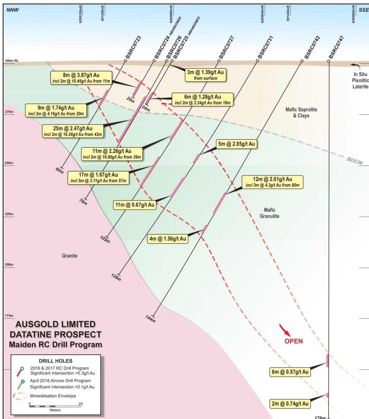
Figure 2. Datatine prospect cross-section showing drill holes, interpreted geology and mineralisation – see Figure 4 for location.
