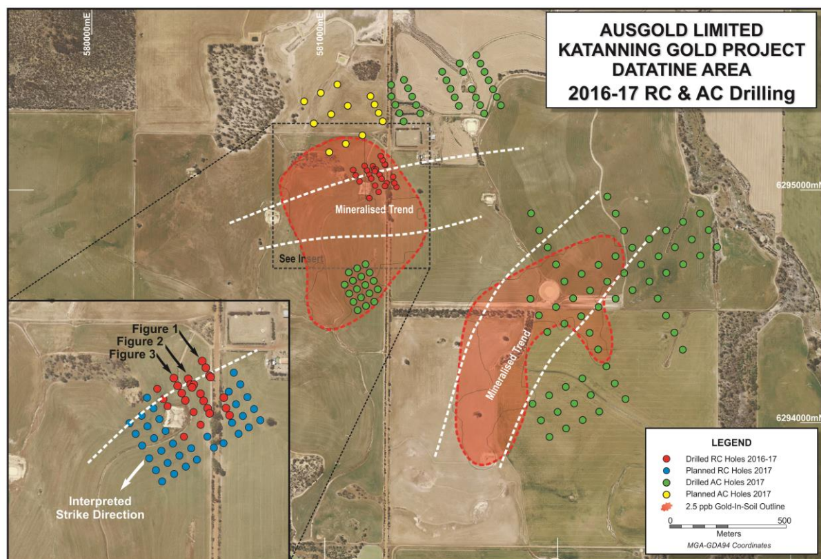
Figure 4. Datatine prospect regional plan showing RC and AC drill holes, interpreted mineralisation
