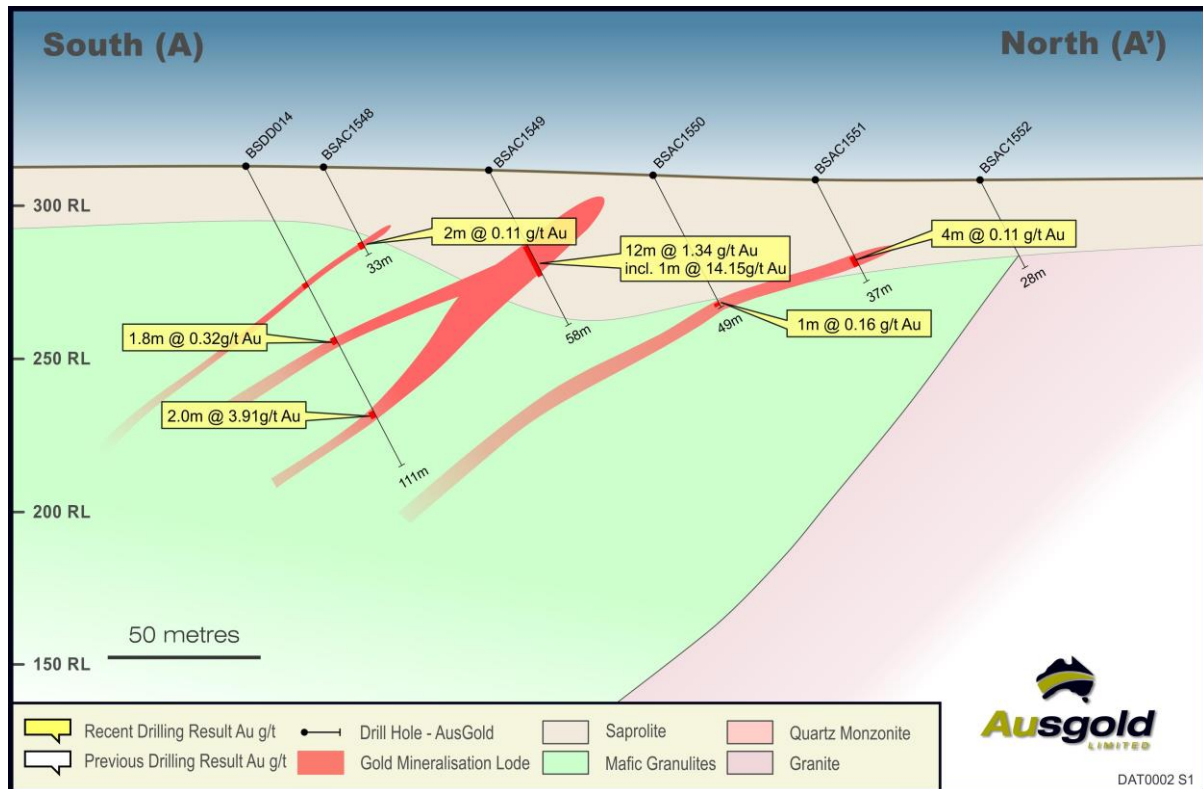
Figure 10 - Cross-section A-A'
