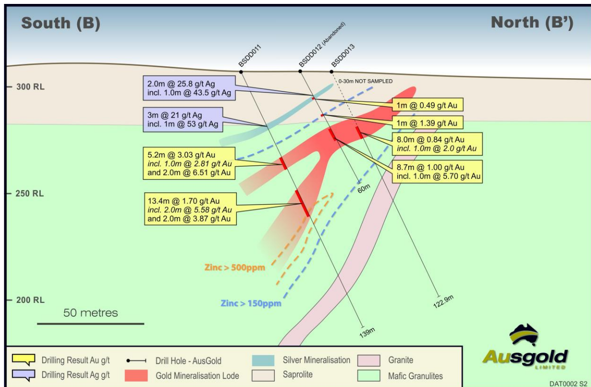
Figure 11 - Cross-section B-B'
