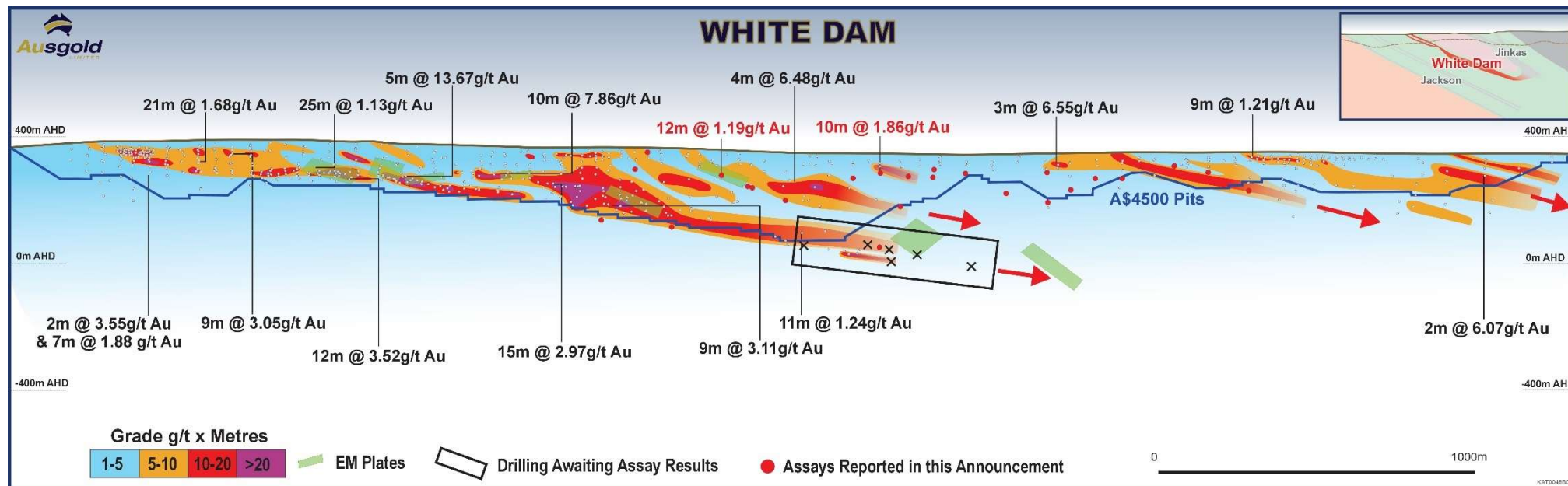
Figure 8 – White Dam trend long-section looking WSW displaying gram-metre contours (0.3g/t Au cut-off), pierce points of existing drilling, DHEM plates, pit optimisation (A$4,500 Resource constraint) and zone where assays are awaiting
