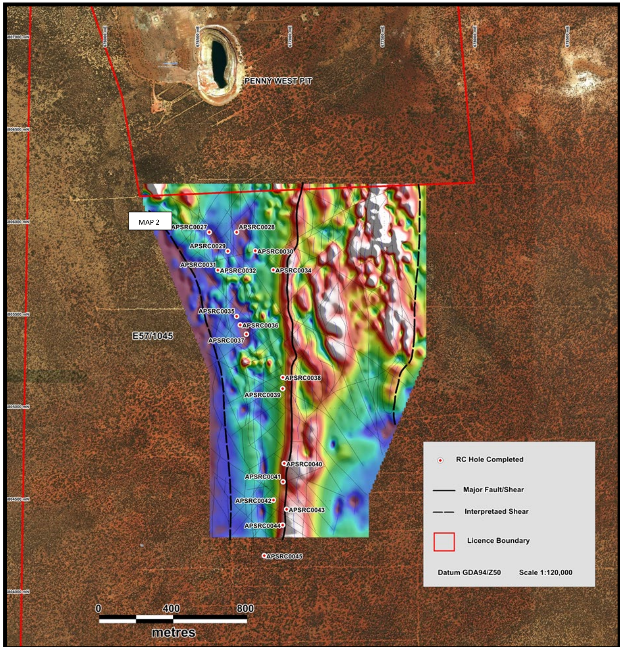
Map 1: Completed drill holes on structural interpretation/ magnetic image. Note the major north-south shear zone (magnetic low) traverses the length of the image and is referred to as the Penny West Shear Zone. The Penny West pit sits in a northwest striking fault and associated shear that splays off this major north-south feature. The northern holes have a similar structural setting to the Penny West deposit.
