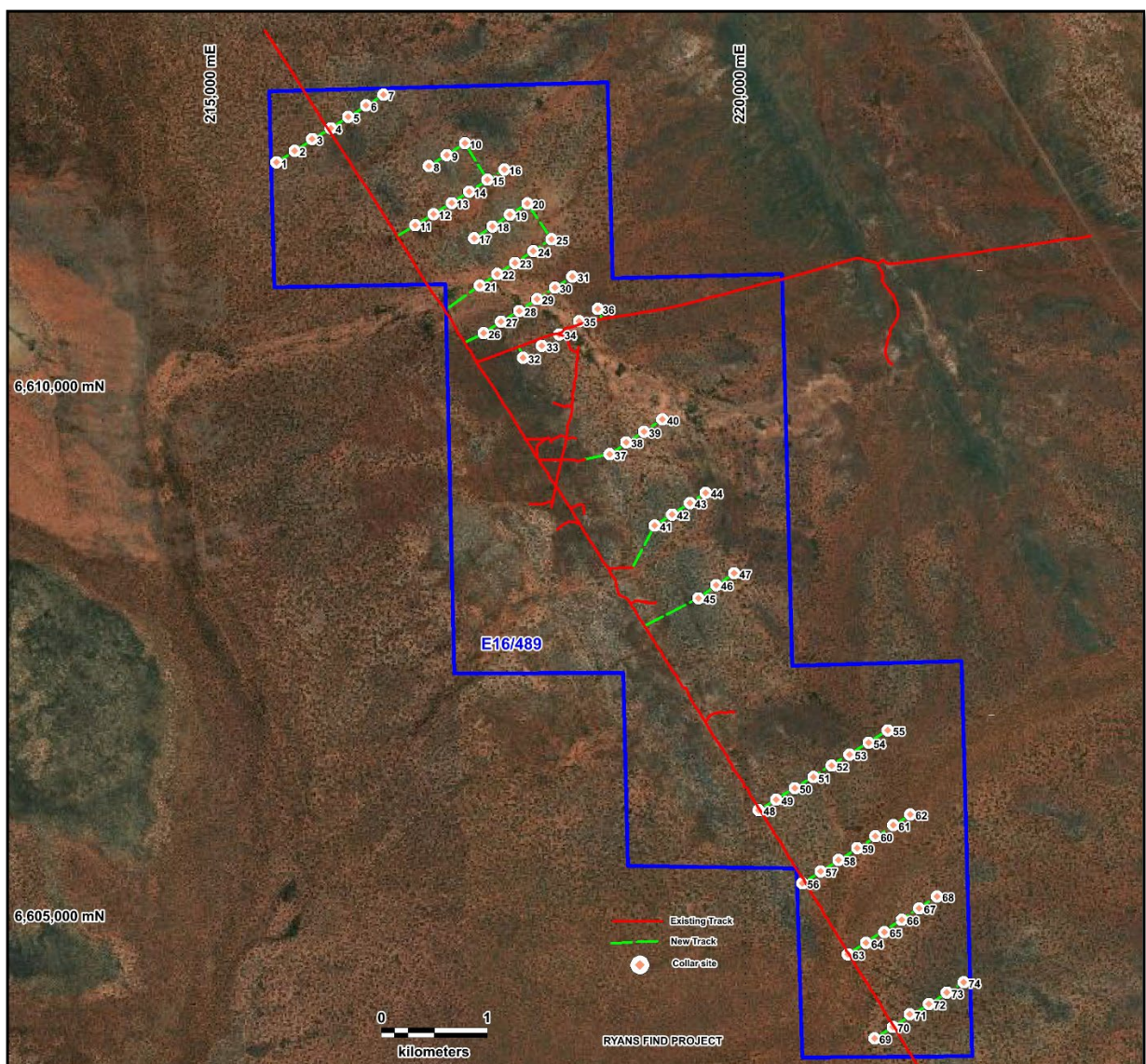
Figure 2: Ryans Find aircore collar plan, the rig started at planned hole 1 on the northern line. Datum MGA94_51.
