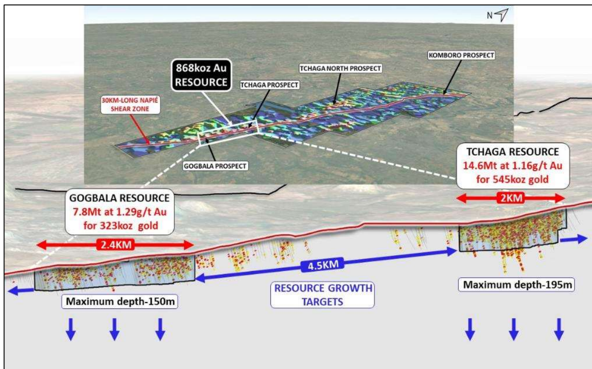
Figure 2: MRE on Tchaga and Gogbala which cover 4.4km of prospective 30km-long Napié Shear Zone
