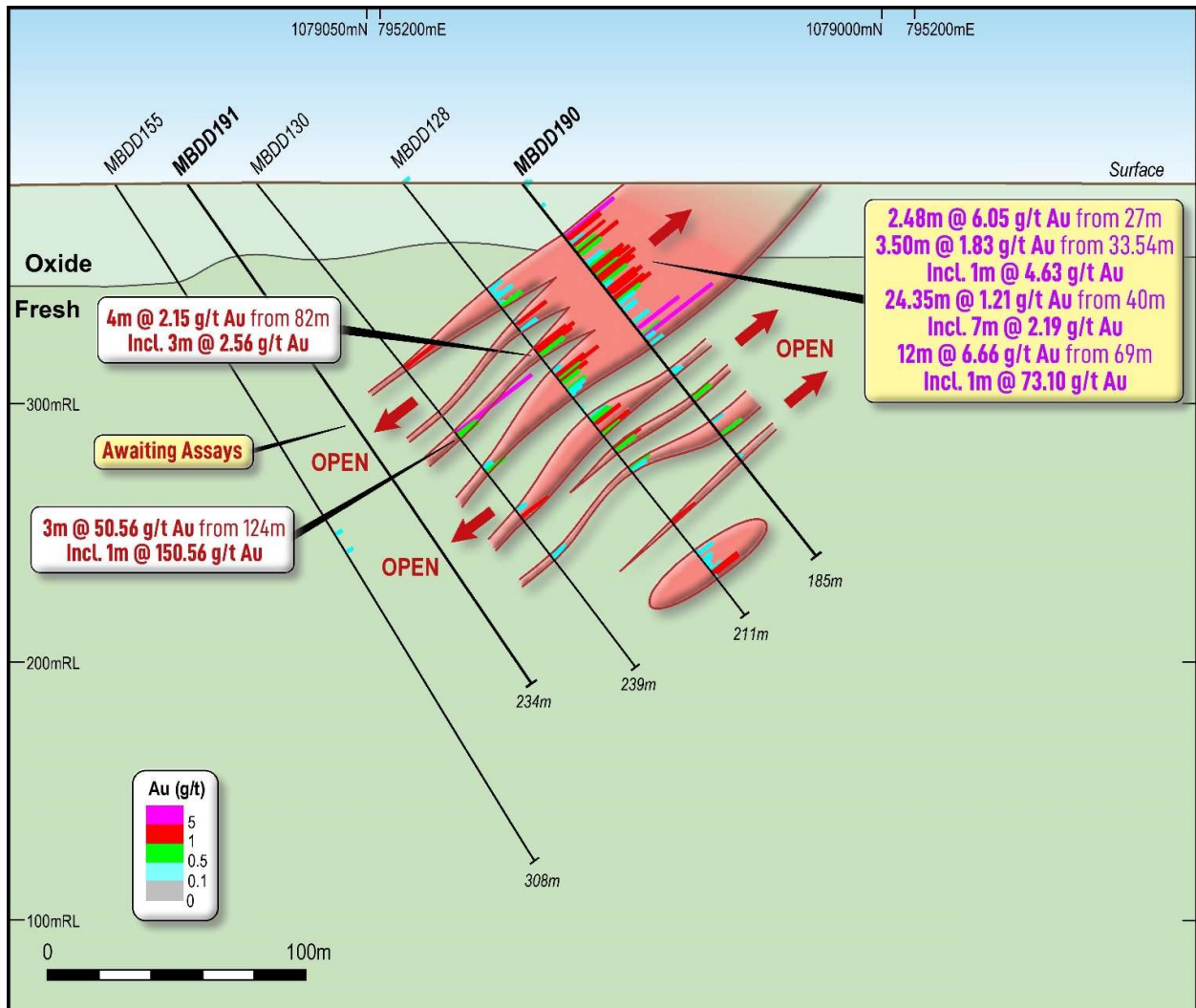
Figure 5: Oblique Cross Section looking northeast (+/-25m) showing new drill results MBDD190 – BM Target 3
