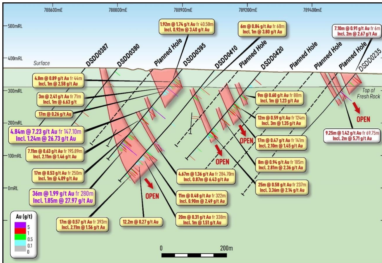
Figure 5: Cross Section looking north (+/-25m) showing new drill results (yellow) for BDT2 10
