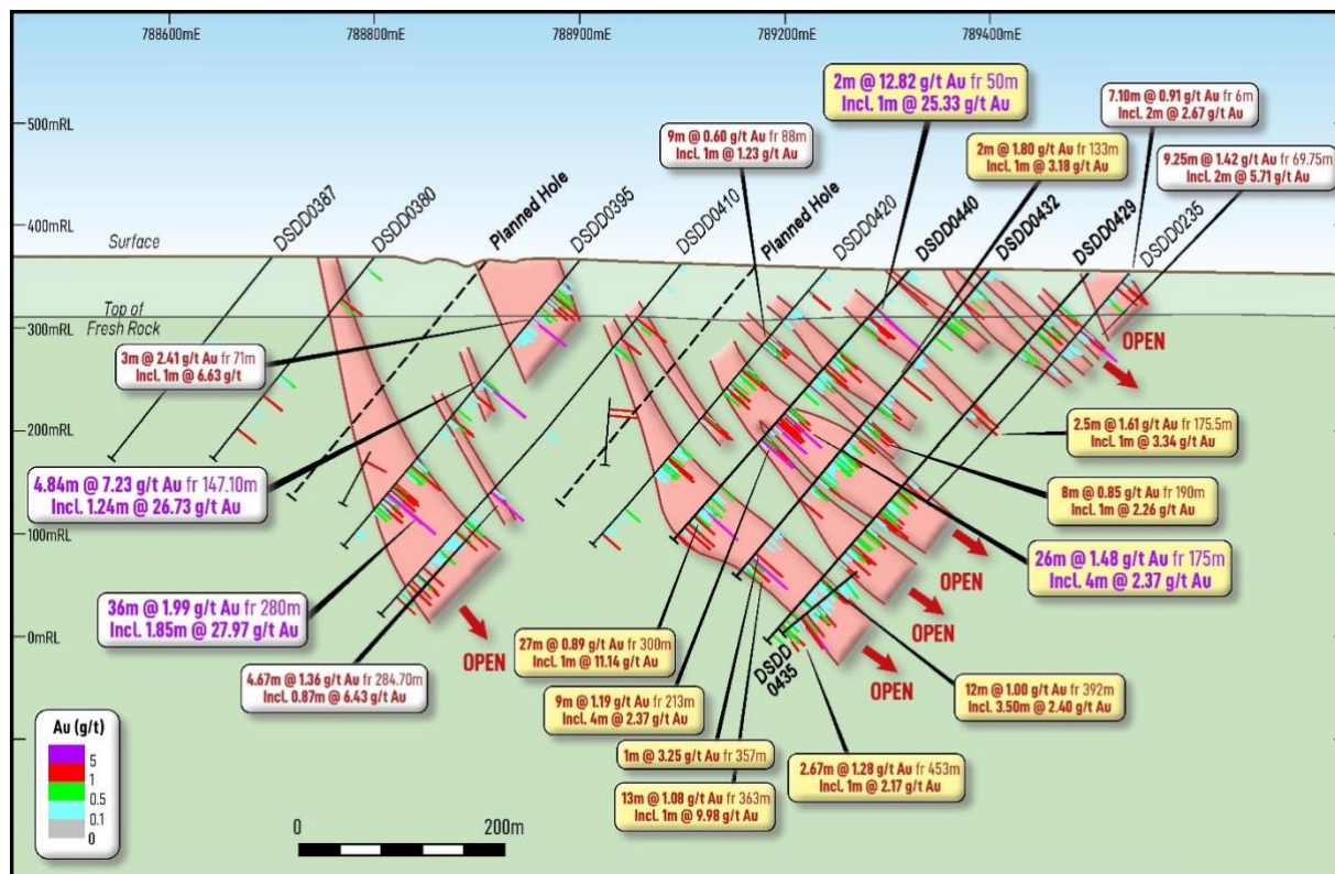
Figure 5: Cross Section looking north (+/-25m) showing new drill results (yellow) for BDT2 12
