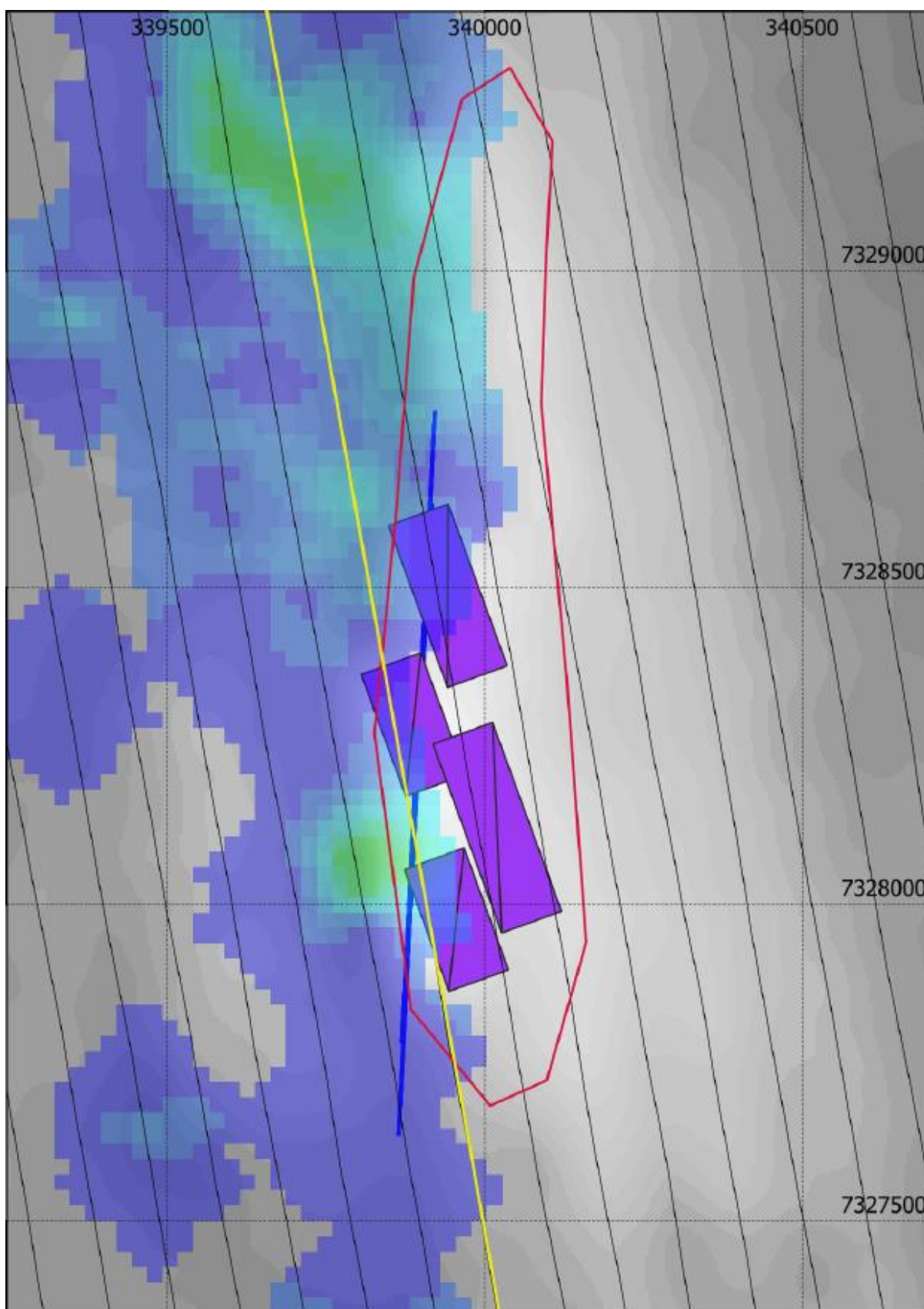
Figure 4. Image of IP effect (colour, transparent) over grey-scale image of channel 30 (0.88 ms) VTEM response and plan view of modelled plate bodies for anomaly ML_03 (red polygon). Map grid lines are 500 m apart. Yellow line shows VTEM line L1160 shown in Figure 5.
