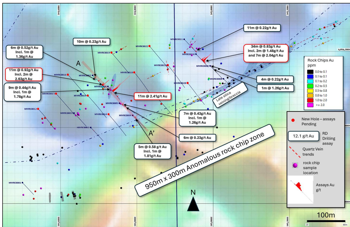
Figure 3 Clifton East plan view showing existing rock chips 1 and recent drill hole traces; latest RC drilling collars shown in red 6 . Background in RTP-TMI magnetic image.
