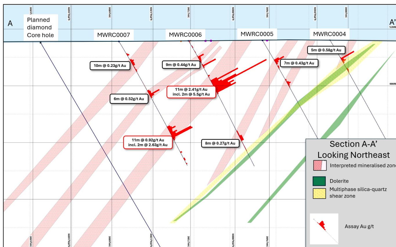
Figure 4 Cross Section A-A' showing location of planned diamond drill hole.
