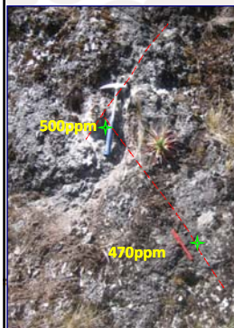
Uranium Anomaly located in Pegmatite Vein
