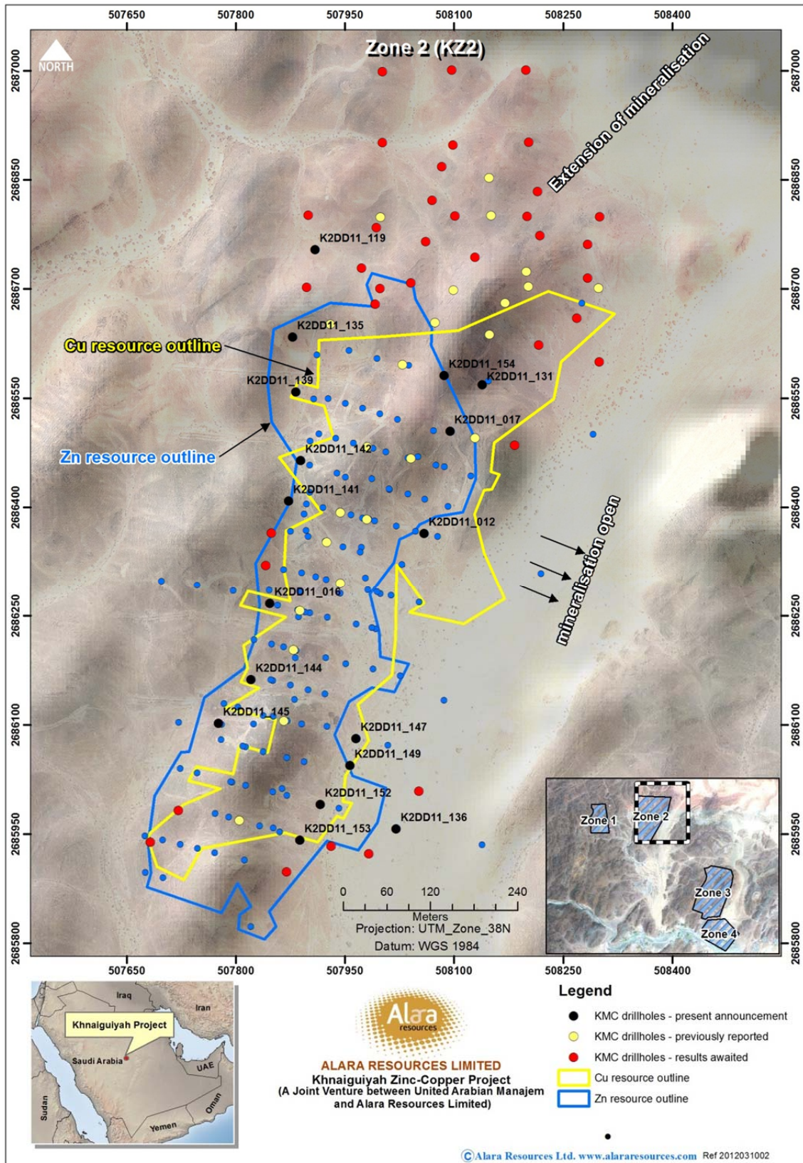
Figure 2: Drill-hole locations in Mineralised Zone 2
