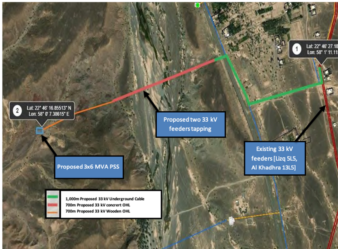
Figure 2: Powerline routes and connection details.
