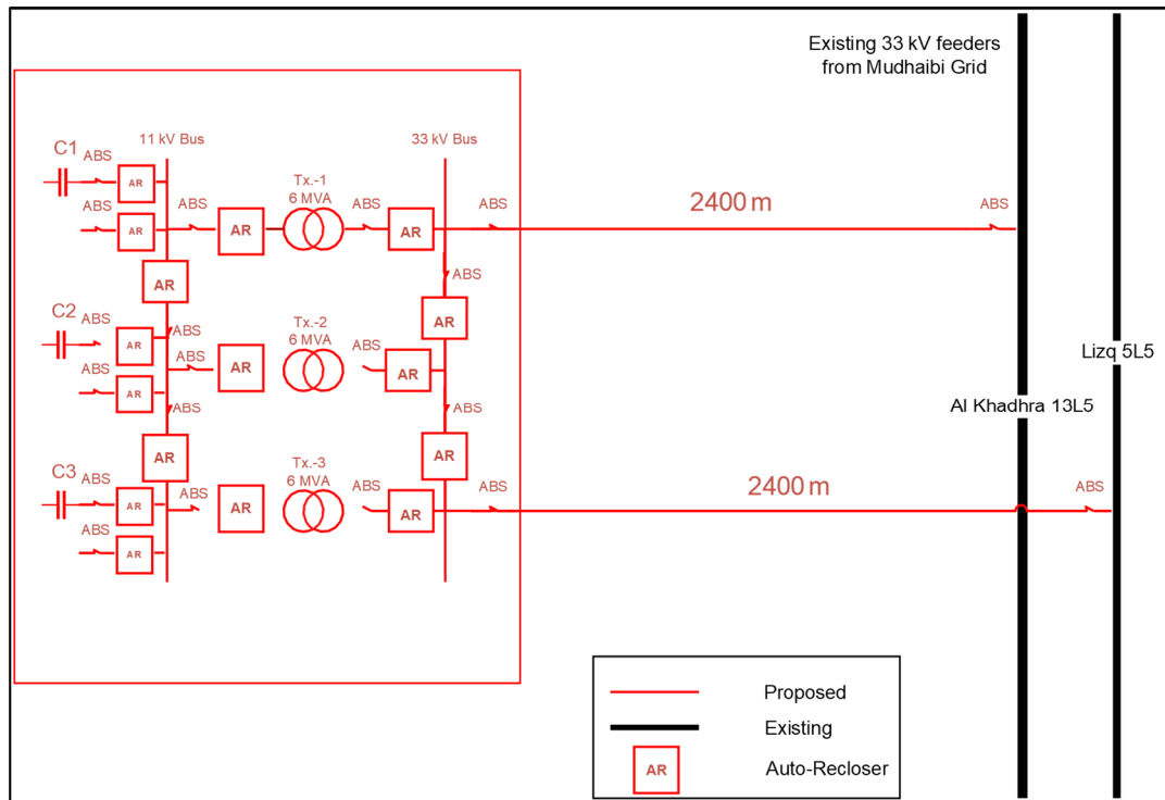
Figure 1 – Connection SLD
