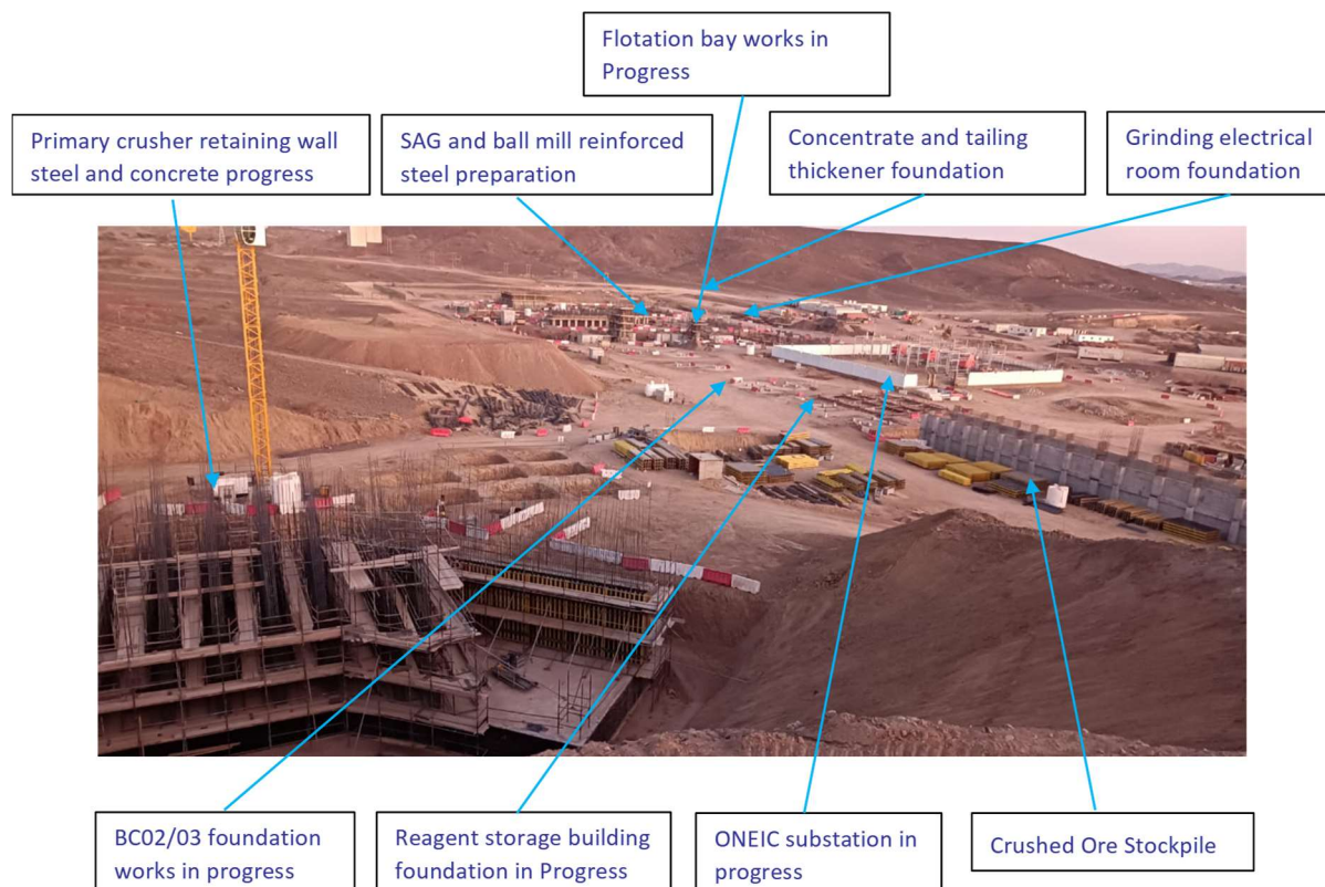
Aerial view of the mine site proper
