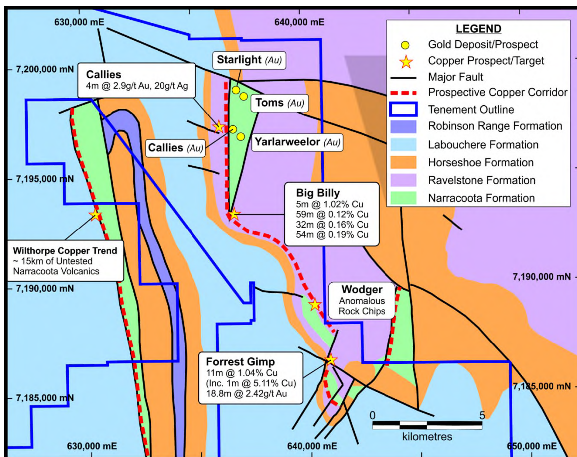
Figure 2: Grosvenor Copper-Gold Project Interpreted Geology Plan
