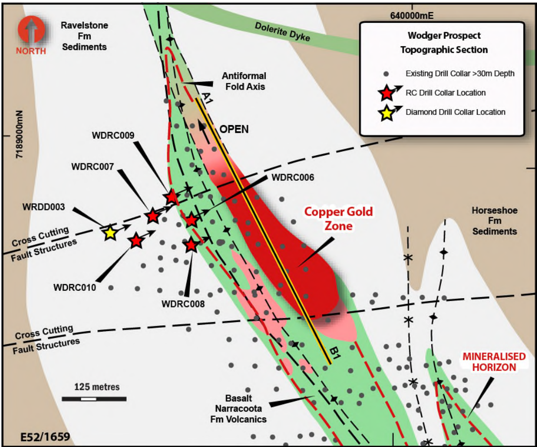
Figure 4: Topographic section showing WDR006-010 and diamond drill collar location in relation to the interpreted geology across the Wodger Prospect plus the >0.1% Cu mineralisation (red) projected to surface.
