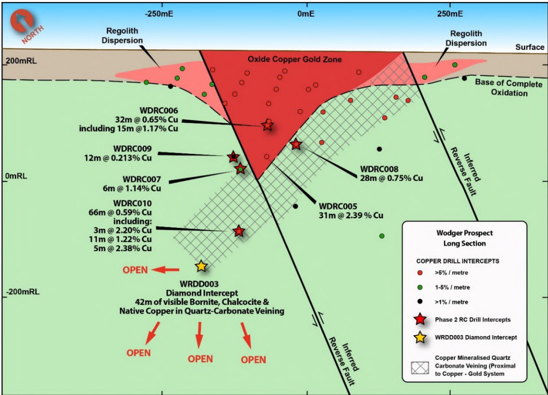
Figure 5: Wodger long section - showing the significant copper intercepts from WDR005-010 in relation to the WRDD003 drill intercept and the maximum copper percent per metre intercepts from previously reported drilling
